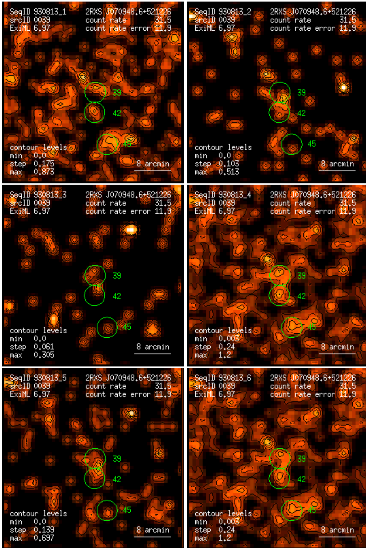
Figure 39: RASS 930813: detection 0039: band rate images, Gaussian filter: (1) PSPC channels 11 – 41, (2) 52 – 90, (3) 91 – 201, (4) 11 – 235, (5) 52 – 201, (6) 11 – 201. Broad band rates in counts/ks. Band rate contour levels in counts/ks/arcmin 2 .
