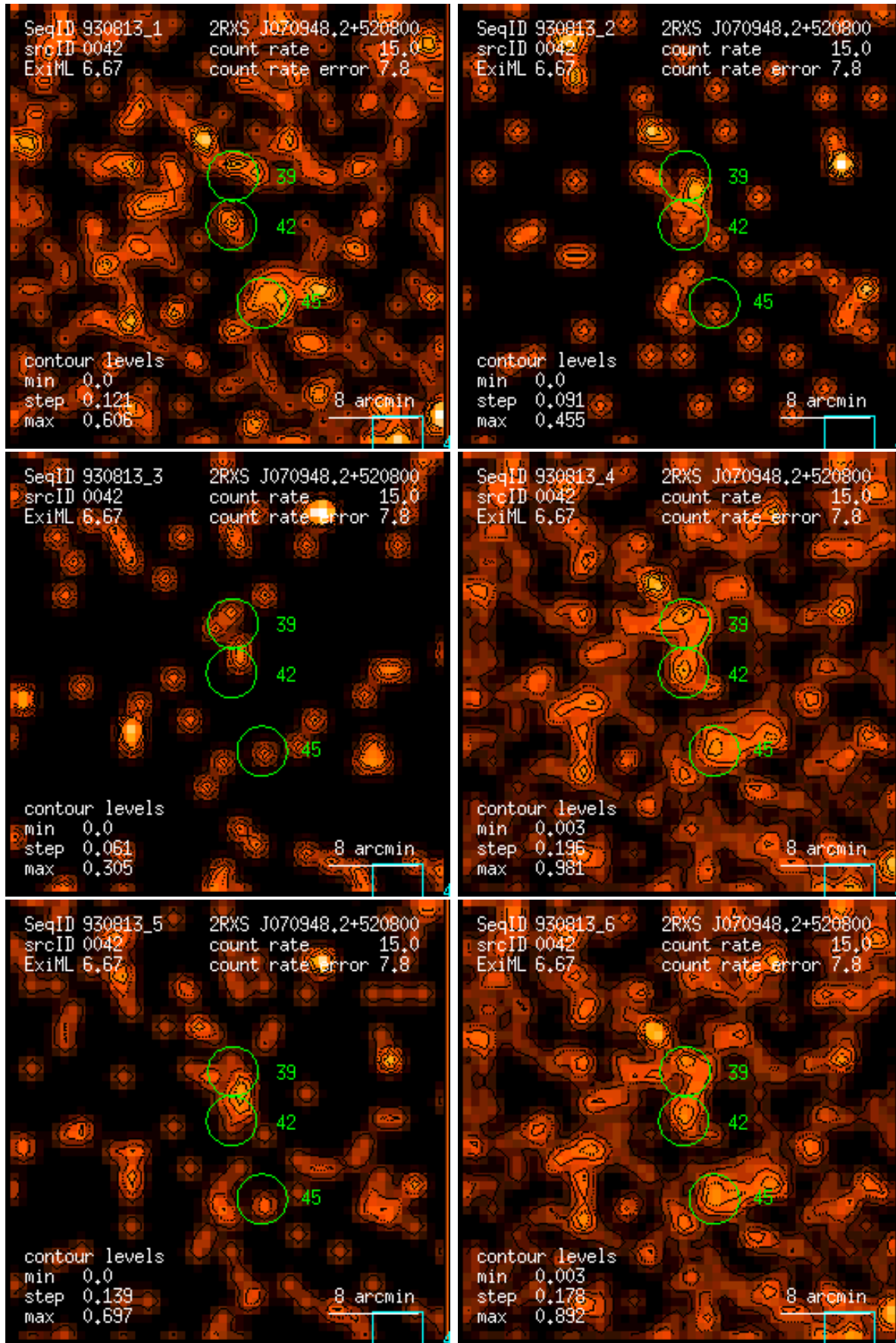
Figure 42: RASS 930813: detection 0042: band rate images, Gaussian filter: (1) PSPC channels 11 – 41, (2) 52 – 90, (3) 91 – 201, (4) 11 – 235, (5) 52 – 201, (6) 11 – 201. Broad band rates in counts/ks. Band rate contour levels in counts/ks/arcmin 2 .
