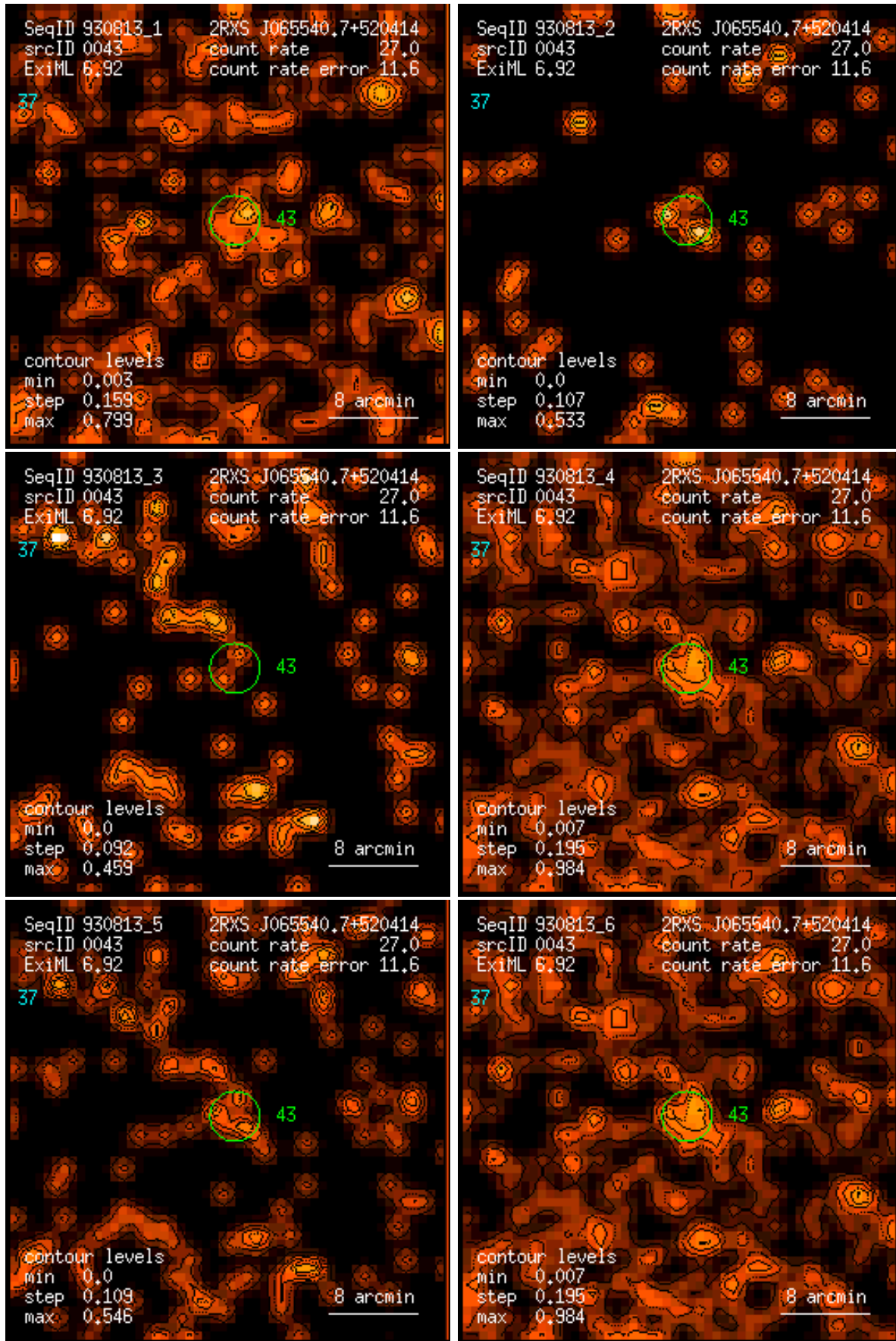
Figure 43: RASS 930813: detection 0043: band rate images, Gaussian filter: (1) PSPC channels 11 – 41, (2) 52 – 90, (3) 91 – 201, (4) 11 – 235, (5) 52 – 201, (6) 11 – 201. Broad band rates in counts/ks. Band rate contour levels in counts/ks/arcmin 2 .
