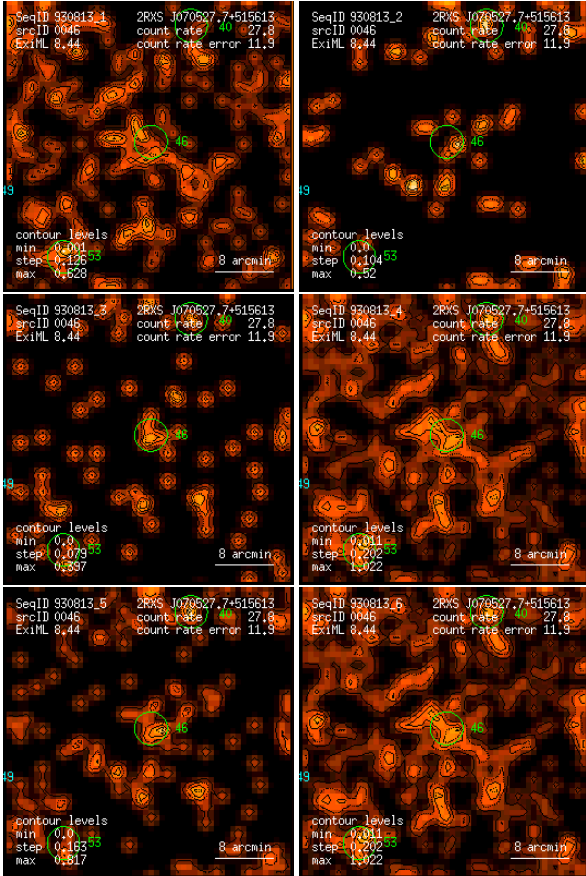
Figure 46: RASS 930813: detection 0046: band rate images, Gaussian filter: (1) PSPC channels 11 – 41, (2) 52 – 90, (3) 91 – 201, (4) 11 – 235, (5) 52 – 201, (6) 11 – 201. Broad band rates in counts/ks. Band rate contour levels in counts/ks/arcmin 2 .
