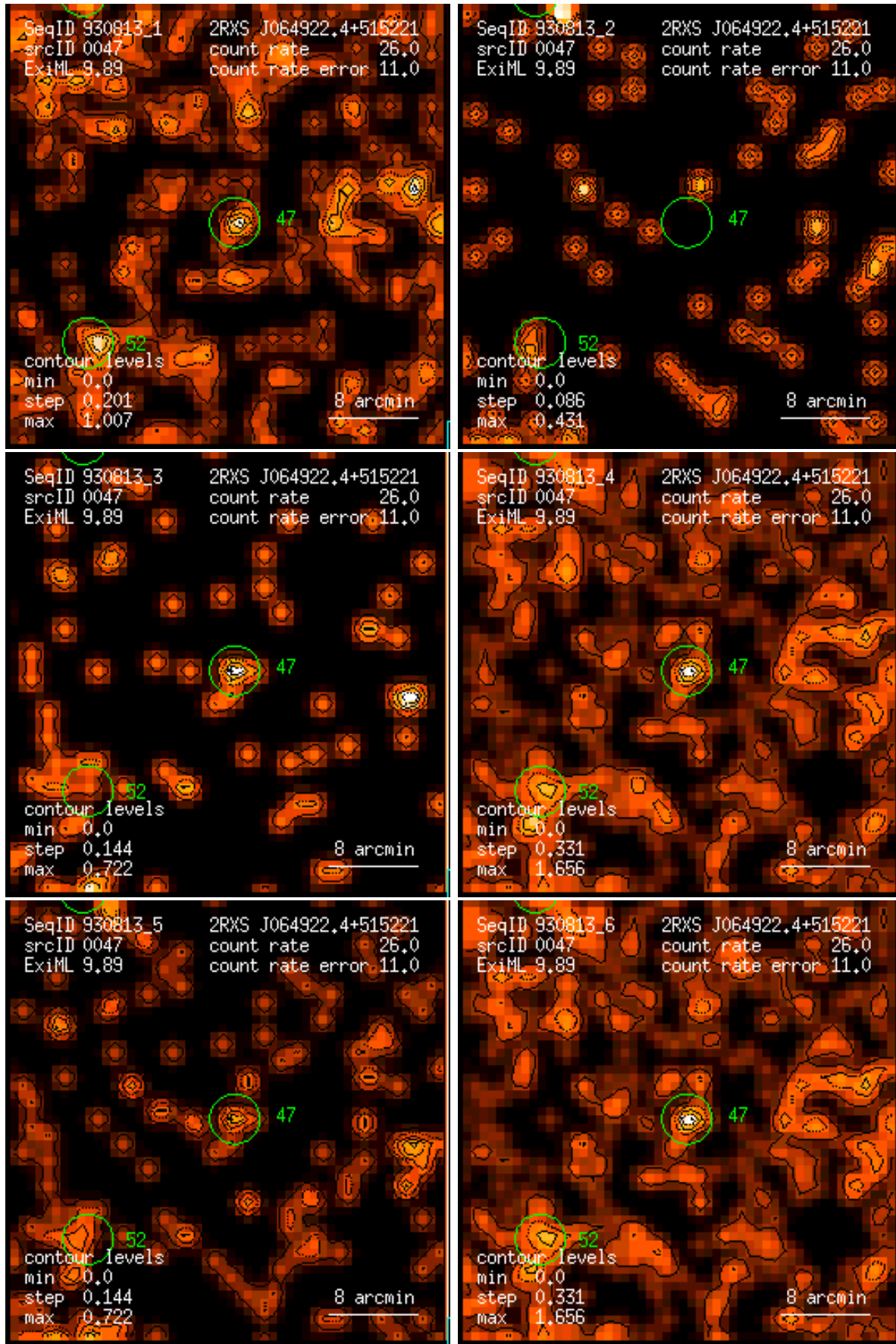
Figure 47: RASS 930813: detection 0047: band rate images, Gaussian filter: (1) PSPC channels 11 – 41, (2) 52 – 90, (3) 91 – 201, (4) 11 – 235, (5) 52 – 201, (6) 11 – 201. Broad band rates in counts/ks. Band rate contour levels in counts/ks/arcmin 2 .
