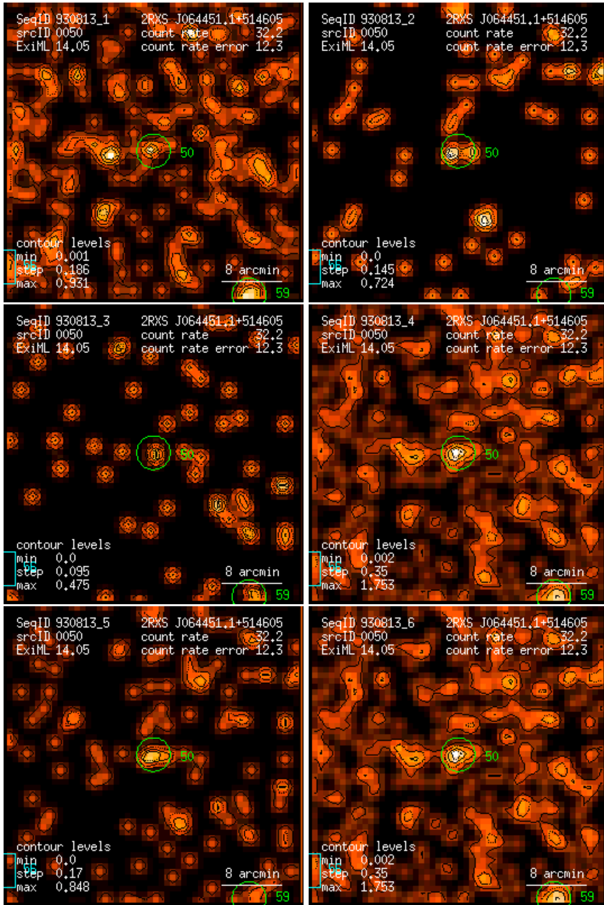
Figure 50: RASS 930813: detection 0050: band rate images, Gaussian filter: (1) PSPC channels 11 – 41, (2) 52 – 90, (3) 91 – 201, (4) 11 – 235, (5) 52 – 201, (6) 11 – 201. Broad band rates in counts/ks. Band rate contour levels in counts/ks/arcmin 2 .
