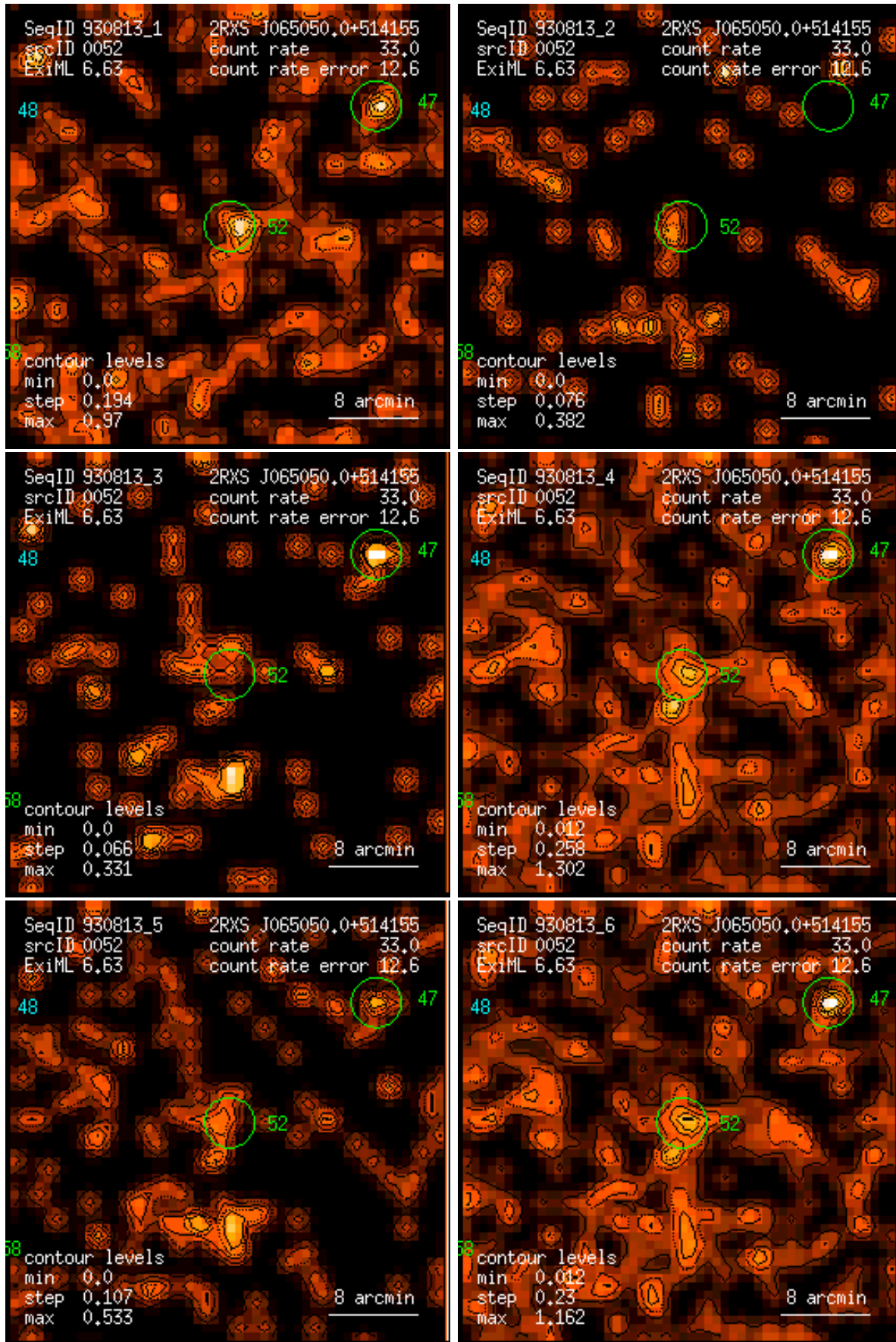
Figure 52: RASS 930813: detection 0052: band rate images, Gaussian filter: (1) PSPC channels 11 – 41, (2) 52 – 90, (3) 91 – 201, (4) 11 – 235, (5) 52 – 201, (6) 11 – 201. Broad band rates in counts/ks. Band rate contour levels in counts/ks/arcmin 2 .
