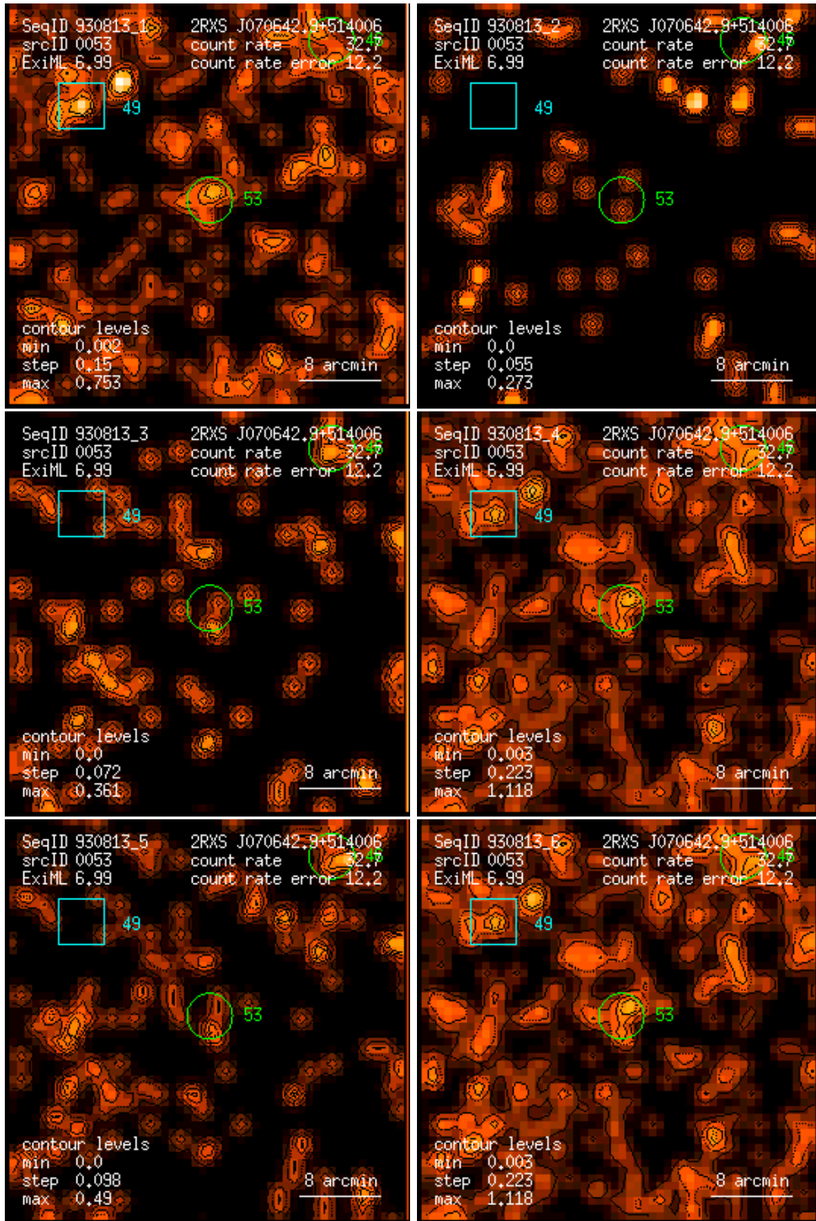
Figure 53: RASS 930813: detection 0053: band rate images, Gaussian filter: (1) PSPC channels 11 – 41, (2) 52 – 90, (3) 91 – 201, (4) 11 – 235, (5) 52 – 201, (6) 11 – 201. Broad band rates in counts/ks. Band rate contour levels in counts/ks/arcmin 2 .
