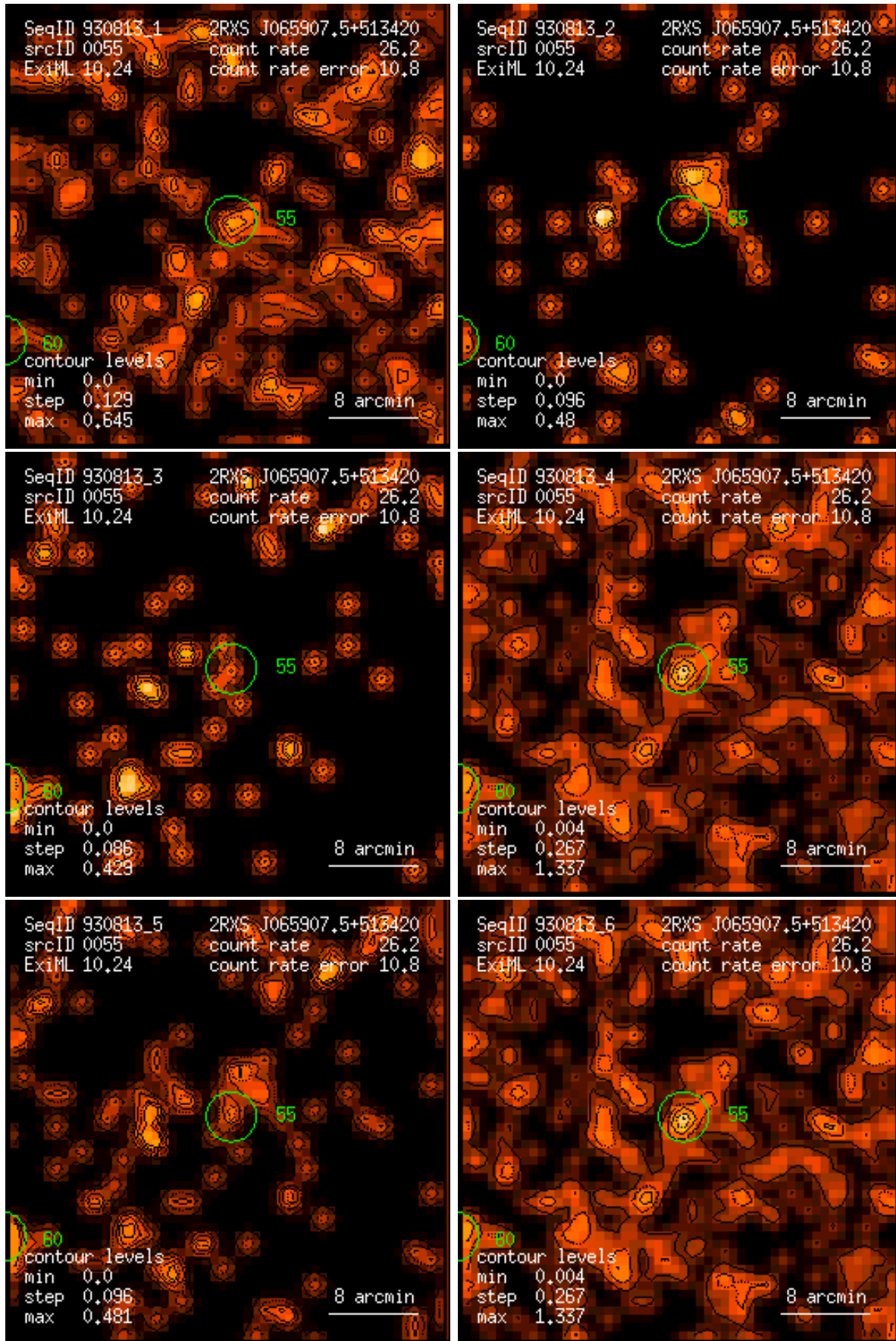
Figure 55: RASS 930813: detection 0055: band rate images, Gaussian filter: (1) PSPC channels 11 – 41, (2) 52 – 90, (3) 91 – 201, (4) 11 – 235, (5) 52 – 201, (6) 11 – 201. Broad band rates in counts/ks. Band rate contour levels in counts/ks/arcmin 2 .
