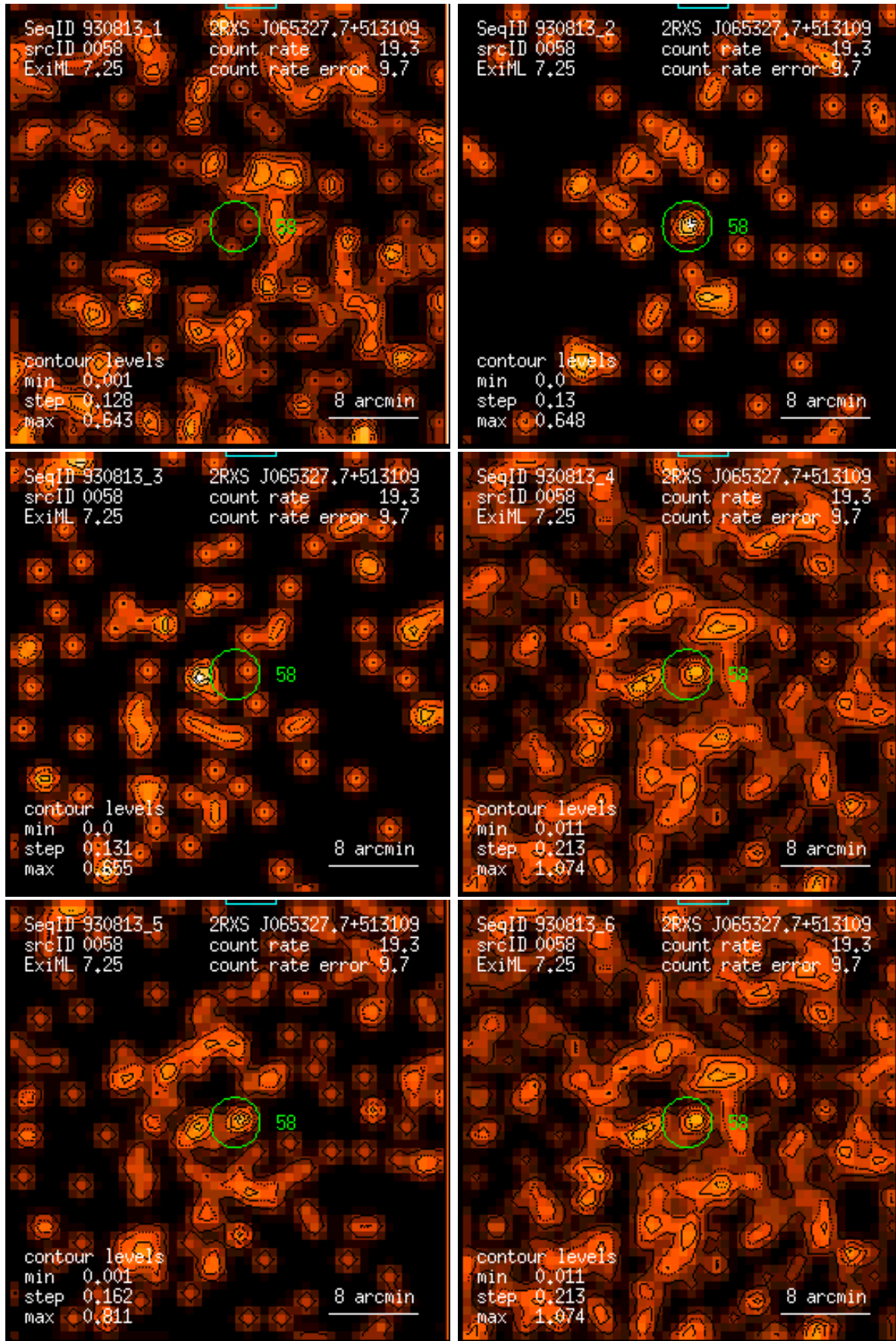
Figure 58: RASS 930813: detection 0058: band rate images, Gaussian filter: (1) PSPC channels 11 – 41, (2) 52 – 90, (3) 91 – 201, (4) 11 – 235, (5) 52 – 201, (6) 11 – 201. Broad band rates in counts/ks. Band rate contour levels in counts/ks/arcmin 2 .
