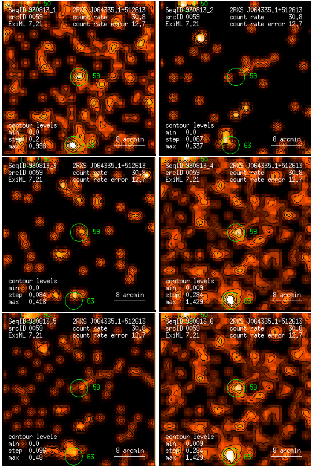
Figure 59: RASS 930813: detection 0059: band rate images, Gaussian filter: (1) PSPC channels 11 – 41, (2) 52 – 90, (3) 91 – 201, (4) 11 – 235, (5) 52 – 201, (6) 11 – 201. Broad band rates in counts/ks. Band rate contour levels in counts/ks/arcmin 2 .
