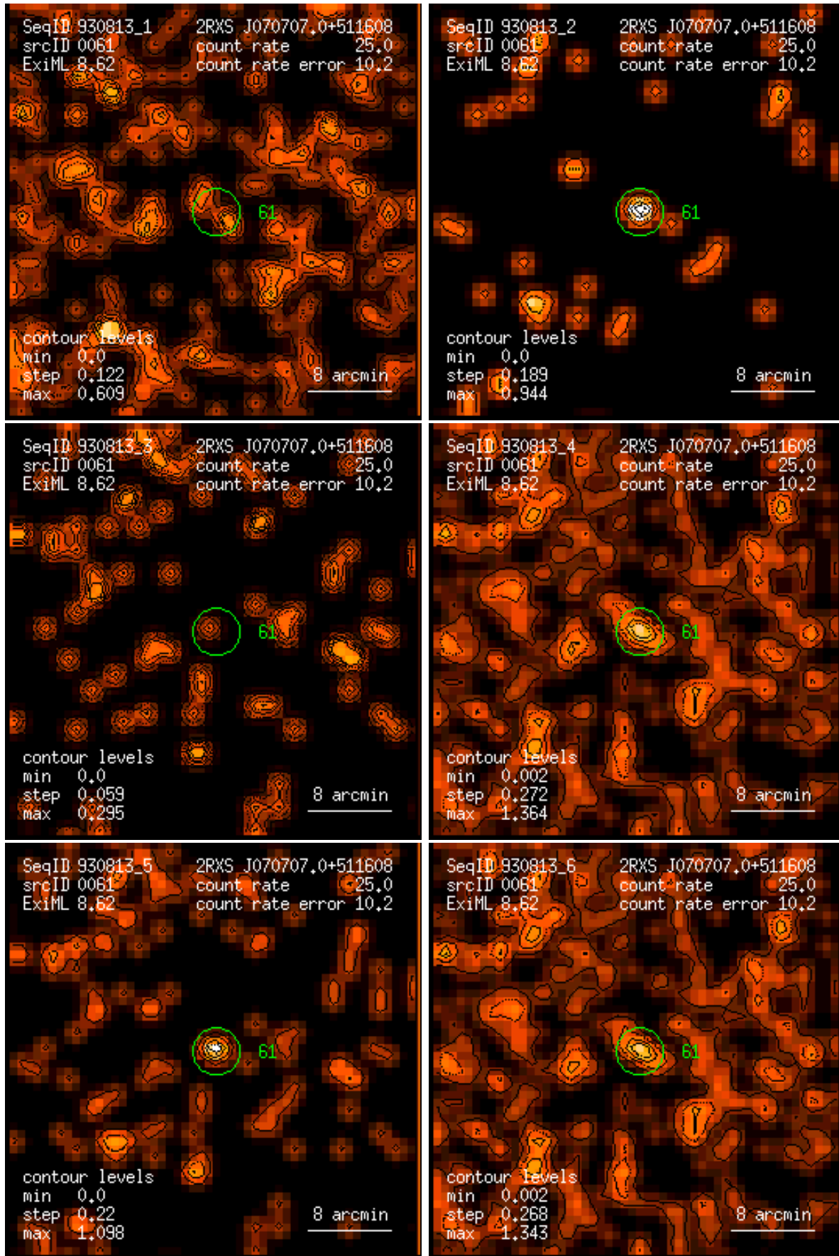
Figure 61: RASS 930813: detection 0061: band rate images, Gaussian filter: (1) PSPC channels 11 – 41, (2) 52 – 90, (3) 91 – 201, (4) 11 – 235, (5) 52 – 201, (6) 11 – 201. Broad band rates in counts/ks. Band rate contour levels in counts/ks/arcmin 2 .
