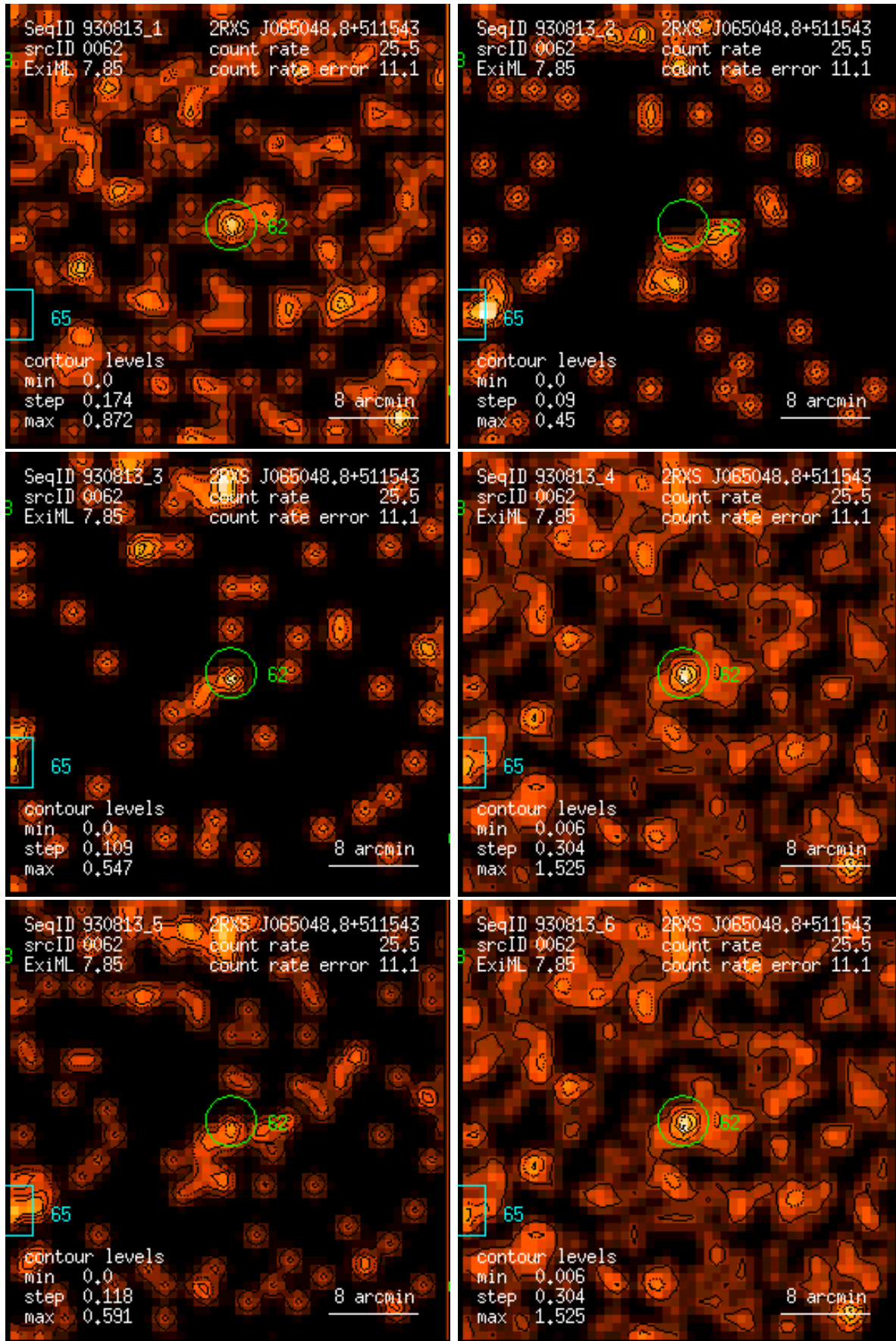
Figure 62: RASS 930813: detection 0062: band rate images, Gaussian filter: (1) PSPC channels 11 – 41, (2) 52 – 90, (3) 91 – 201, (4) 11 – 235, (5) 52 – 201, (6) 11 – 201. Broad band rates in counts/ks. Band rate contour levels in counts/ks/arcmin 2 .
