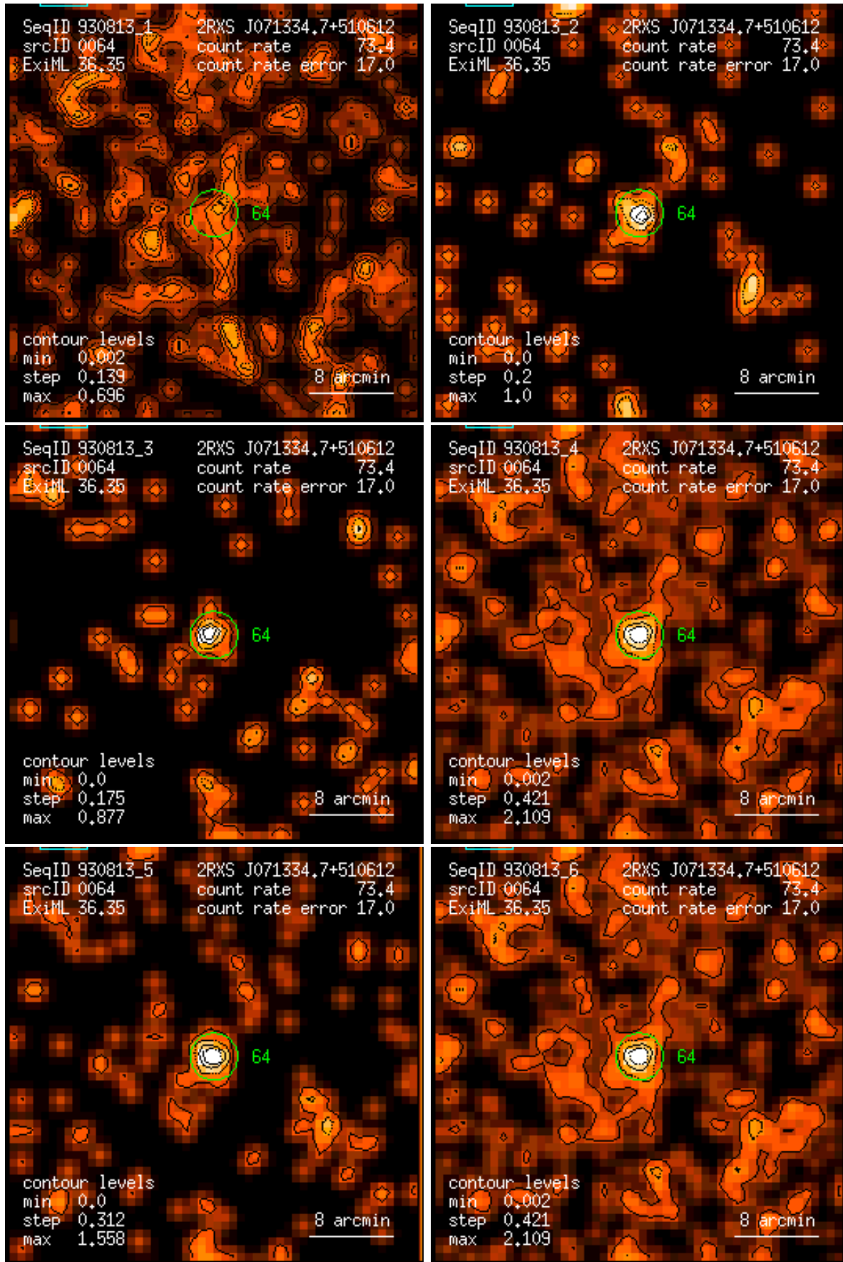
Figure 64: RASS 930813: detection 0064: band rate images, Gaussian filter: (1) PSPC channels 11 – 41, (2) 52 – 90, (3) 91 – 201, (4) 11 – 235, (5) 52 – 201, (6) 11 – 201. Broad band rates in counts/ks. Band rate contour levels in counts/ks/arcmin 2 .
