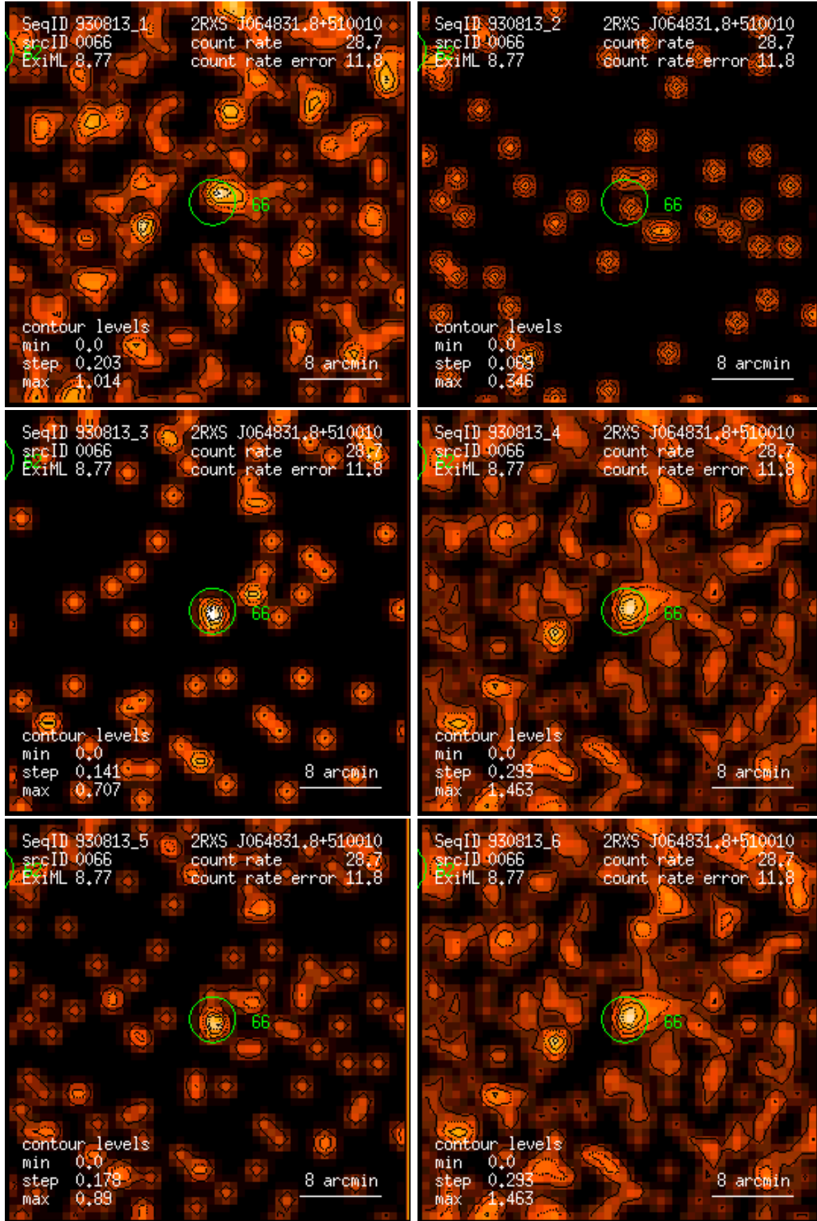
Figure 66: RASS 930813: detection 0066: band rate images, Gaussian filter: (1) PSPC channels 11 – 41, (2) 52 – 90, (3) 91 – 201, (4) 11 – 235, (5) 52 – 201, (6) 11 – 201. Broad band rates in counts/ks. Band rate contour levels in counts/ks/arcmin 2 .
