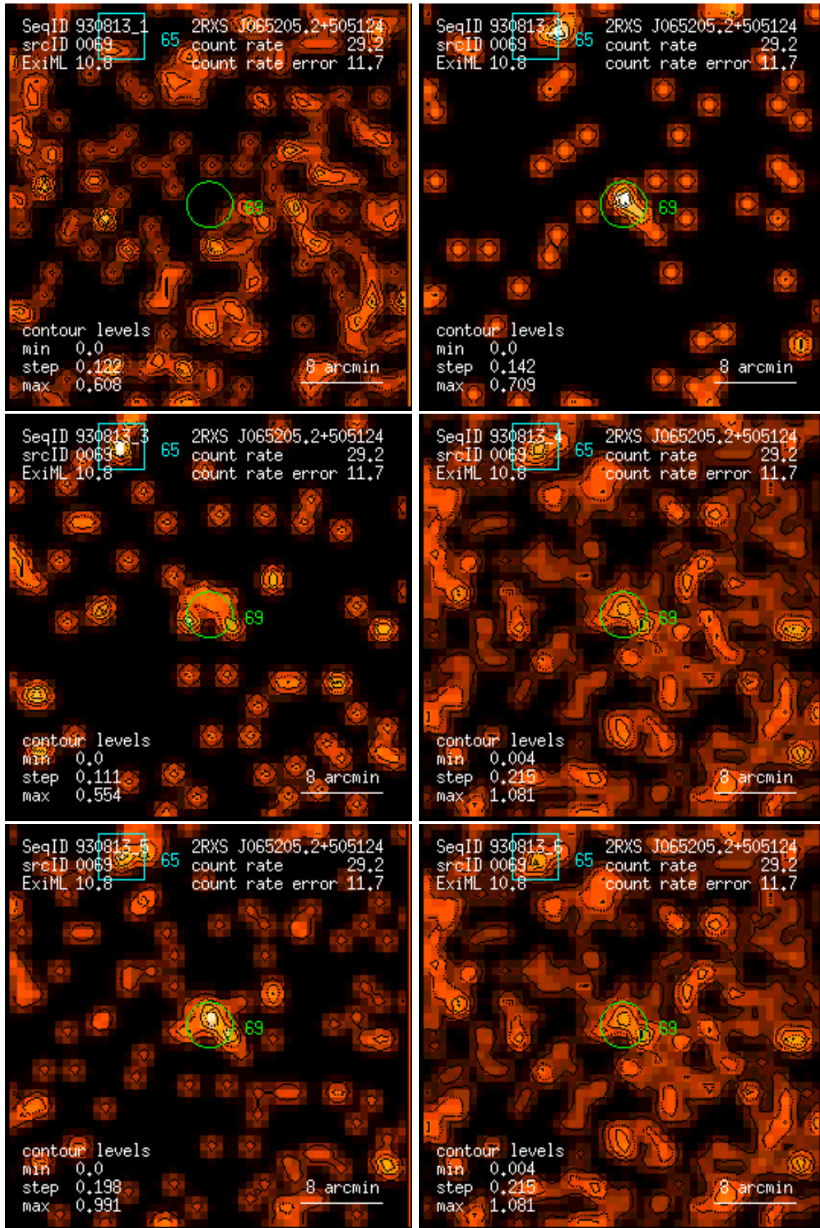
Figure 69: RASS 930813: detection 0069: band rate images, Gaussian filter: (1) PSPC channels 11 – 41, (2) 52 – 90, (3) 91 – 201, (4) 11 – 235, (5) 52 – 201, (6) 11 – 201. Broad band rates in counts/ks. Band rate contour levels in counts/ks/arcmin 2 .
