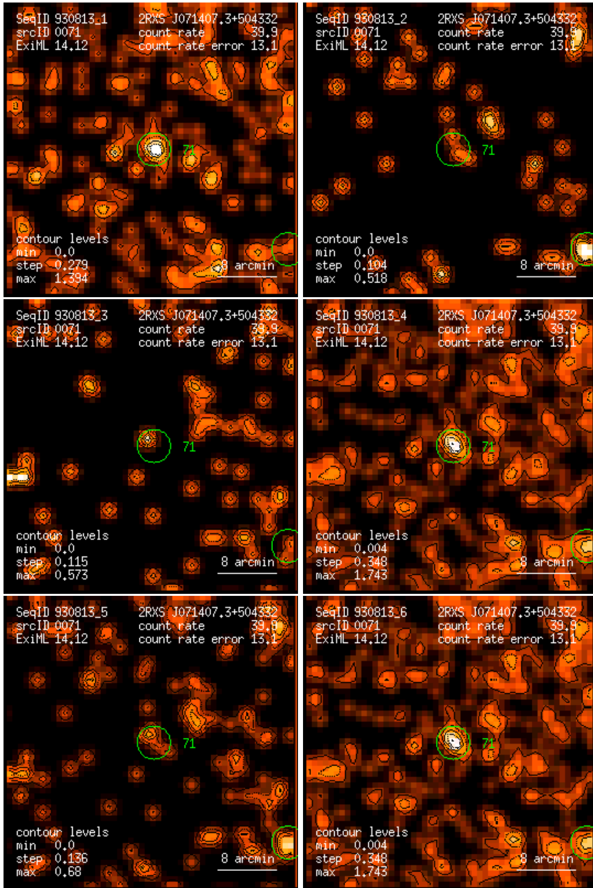
Figure 71: RASS 930813: detection 0071: band rate images, Gaussian filter: (1) PSPC channels 11 – 41, (2) 52 – 90, (3) 91 – 201, (4) 11 – 235, (5) 52 – 201, (6) 11 – 201. Broad band rates in counts/ks. Band rate contour levels in counts/ks/arcmin 2 .
