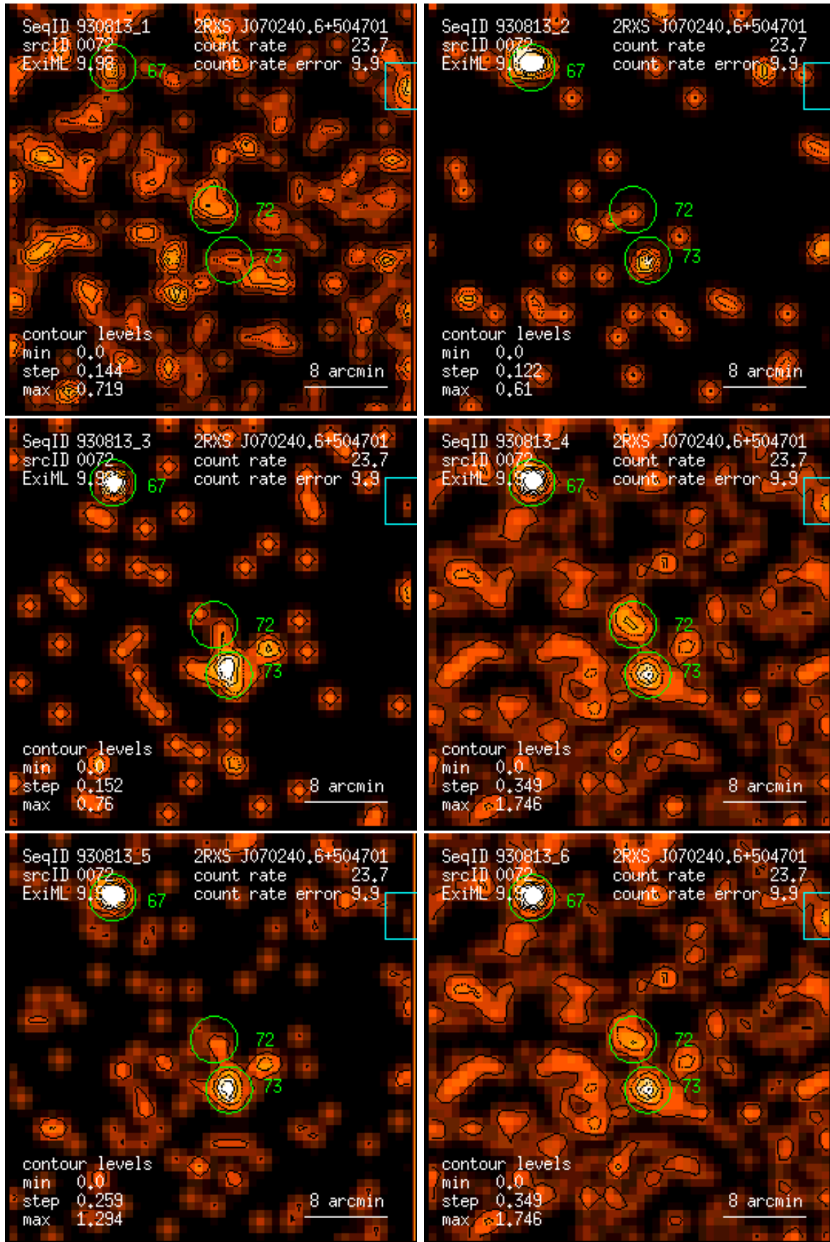
Figure 72: RASS 930813: detection 0072: band rate images, Gaussian filter: (1) PSPC channels 11 – 41, (2) 52 – 90, (3) 91 – 201, (4) 11 – 235, (5) 52 – 201, (6) 11 – 201. Broad band rates in counts/ks. Band rate contour levels in counts/ks/arcmin 2 .
