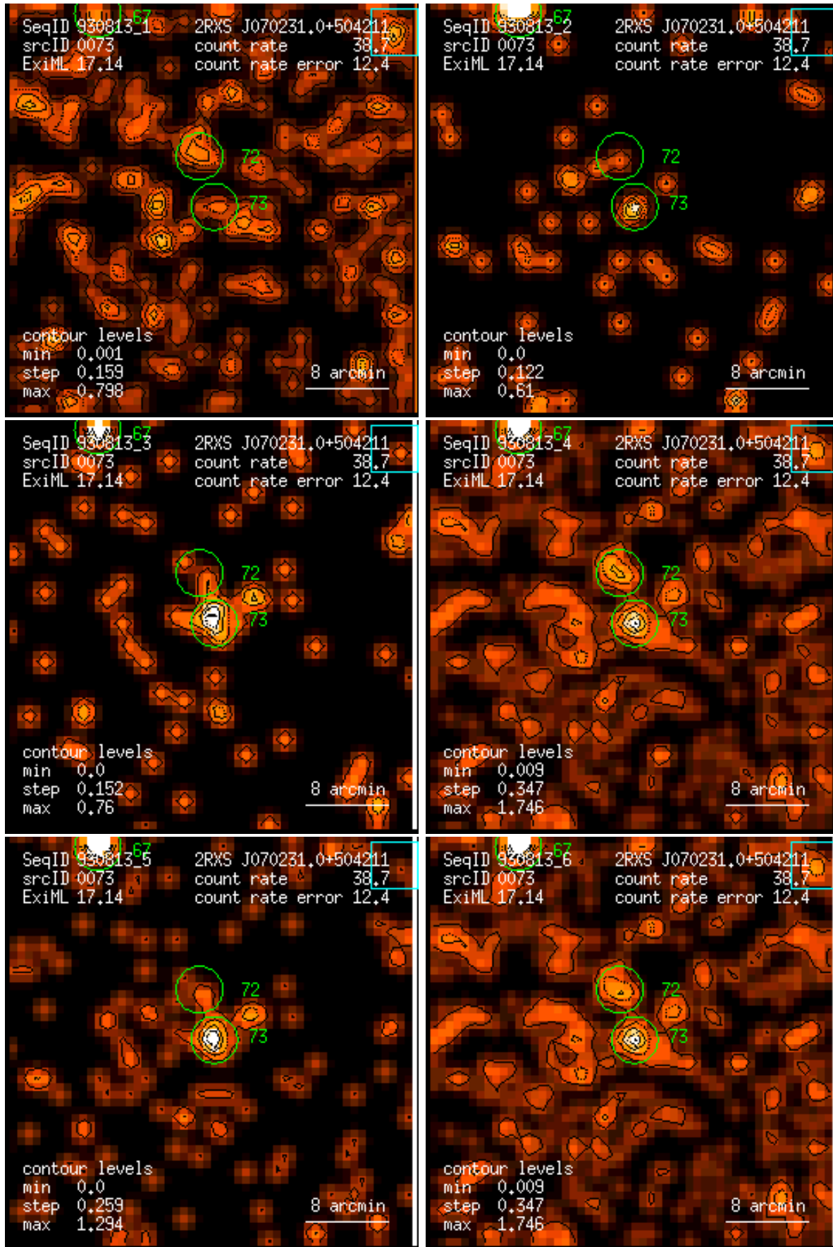
Figure 73: RASS 930813: detection 0073: band rate images, Gaussian filter: (1) PSPC channels 11 – 41, (2) 52 – 90, (3) 91 – 201, (4) 11 – 235, (5) 52 – 201, (6) 11 – 201. Broad band rates in counts/ks. Band rate contour levels in counts/ks/arcmin 2 .
