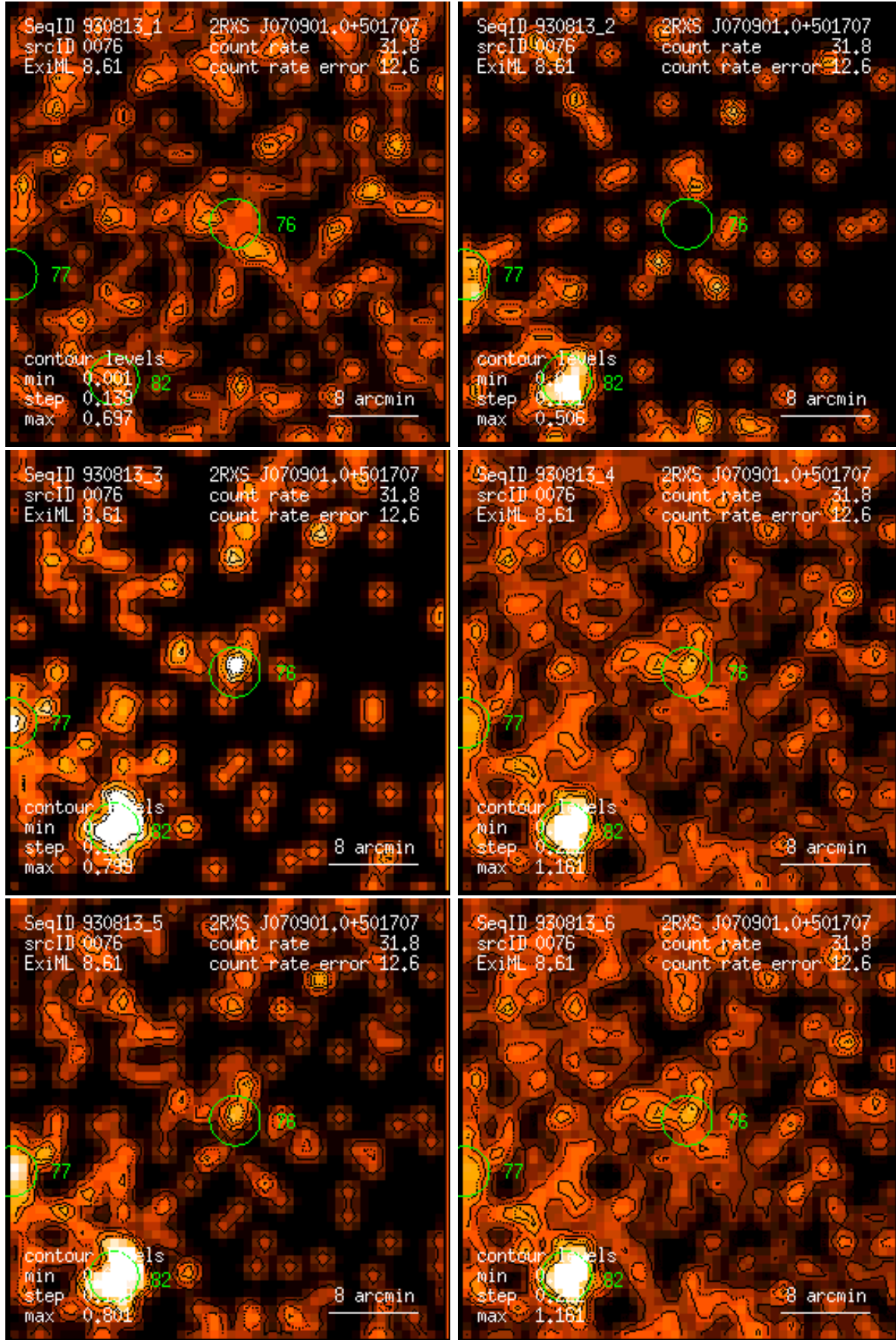
Figure 76: RASS 930813: detection 0076: band rate images, Gaussian filter: (1) PSPC channels 11 – 41, (2) 52 – 90, (3) 91 – 201, (4) 11 – 235, (5) 52 – 201, (6) 11 – 201. Broad band rates in counts/ks. Band rate contour levels in counts/ks/arcmin 2 .
