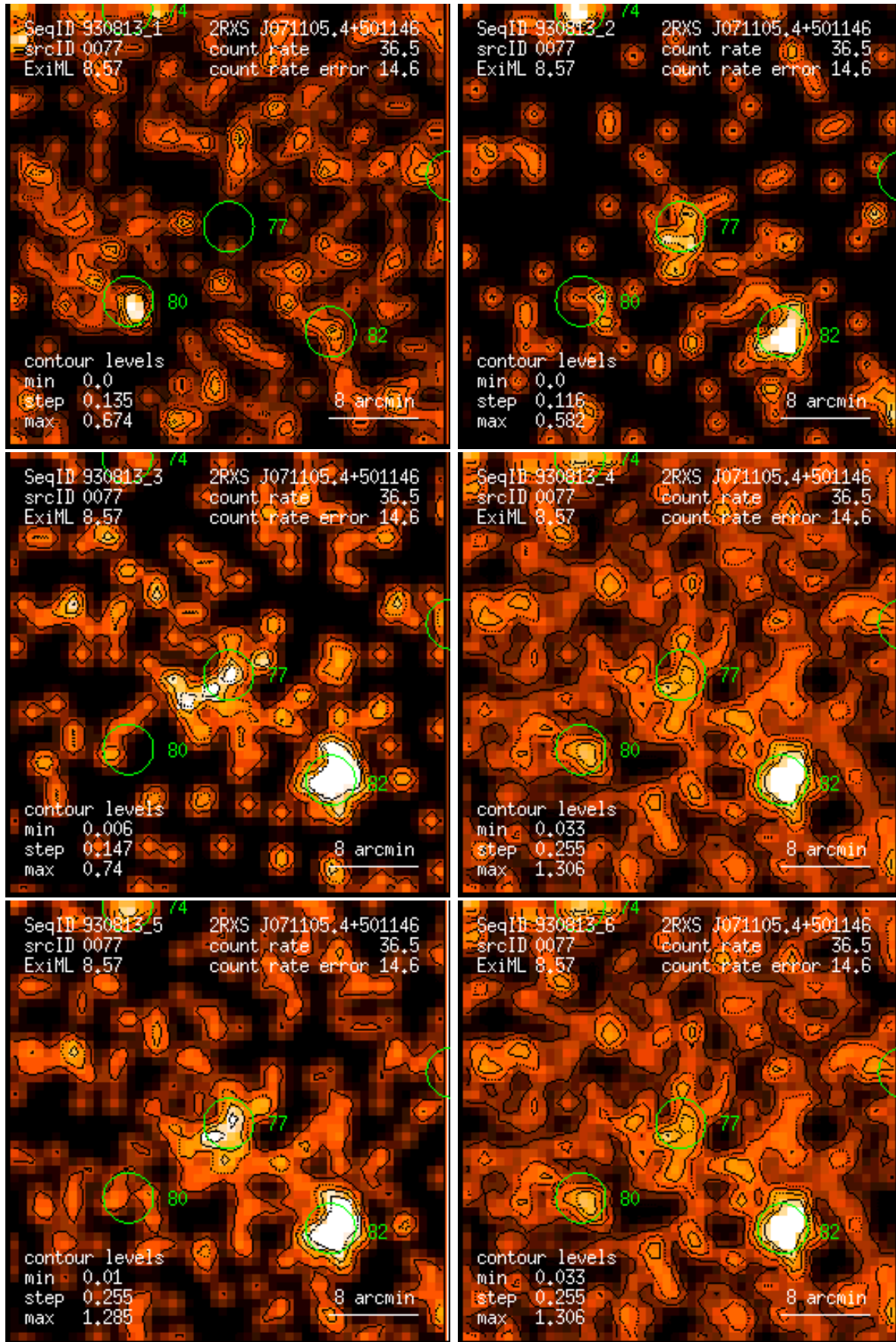
Figure 77: RASS 930813: detection 0077: band rate images, Gaussian filter: (1) PSPC channels 11 – 41, (2) 52 – 90, (3) 91 – 201, (4) 11 – 235, (5) 52 – 201, (6) 11 – 201. Broad band rates in counts/ks. Band rate contour levels in counts/ks/arcmin 2 .
