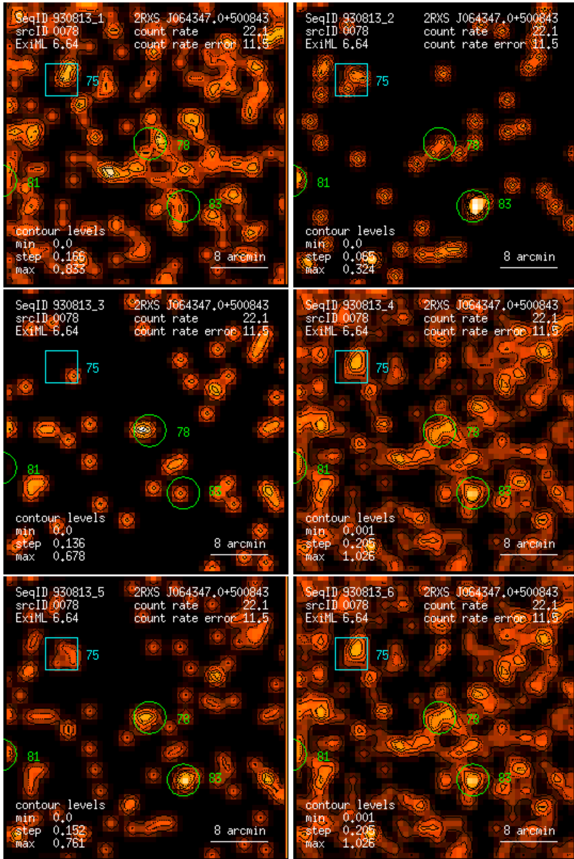
Figure 78: RASS 930813: detection 0078: band rate images, Gaussian filter: (1) PSPC channels 11 – 41, (2) 52 – 90, (3) 91 – 201, (4) 11 – 235, (5) 52 – 201, (6) 11 – 201. Broad band rates in counts/ks. Band rate contour levels in counts/ks/arcmin 2 .
