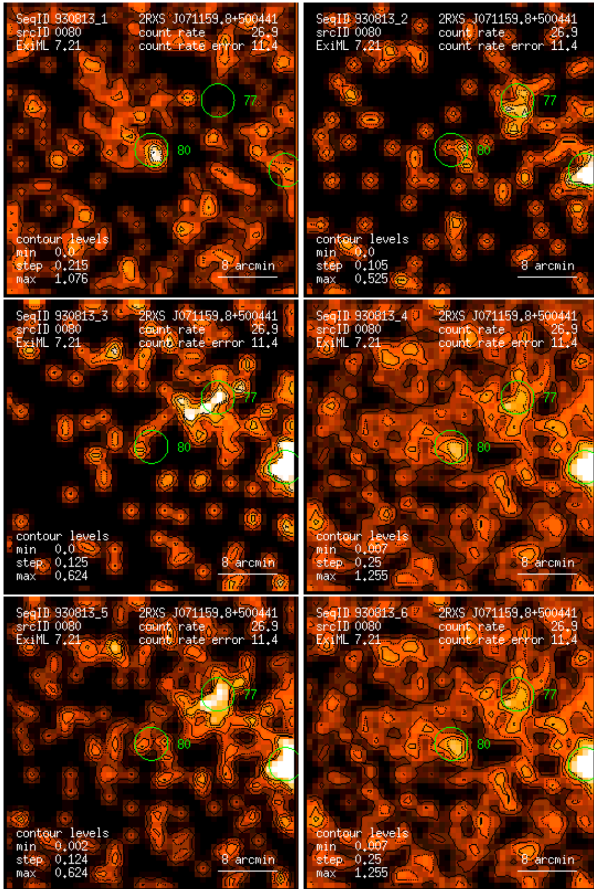
Figure 80: RASS 930813: detection 0080: band rate images, Gaussian filter: (1) PSPC channels 11 – 41, (2) 52 – 90, (3) 91 – 201, (4) 11 – 235, (5) 52 – 201, (6) 11 – 201. Broad band rates in counts/ks. Band rate contour levels in counts/ks/arcmin 2 .
