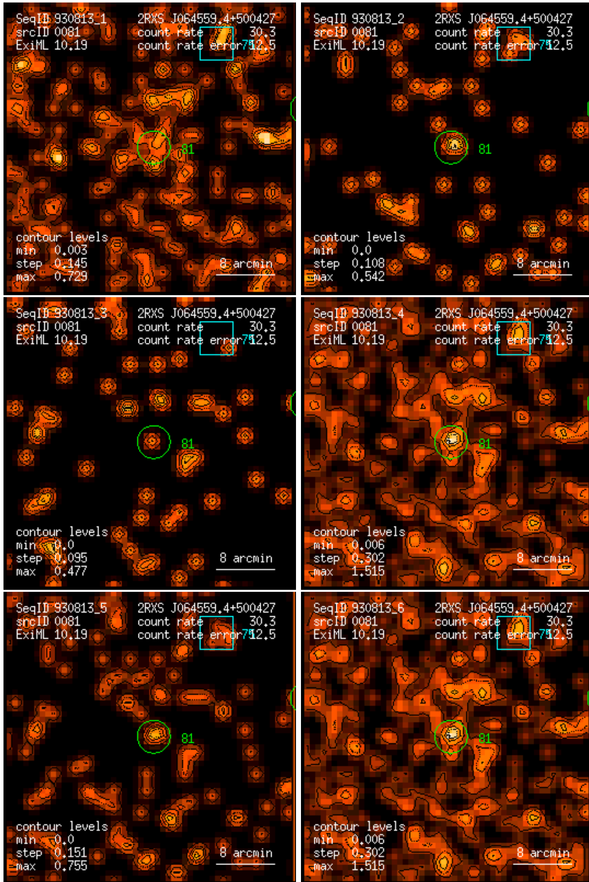
Figure 81: RASS 930813: detection 0081: band rate images, Gaussian filter: (1) PSPC channels 11 – 41, (2) 52 – 90, (3) 91 – 201, (4) 11 – 235, (5) 52 – 201, (6) 11 – 201. Broad band rates in counts/ks. Band rate contour levels in counts/ks/arcmin 2 .
