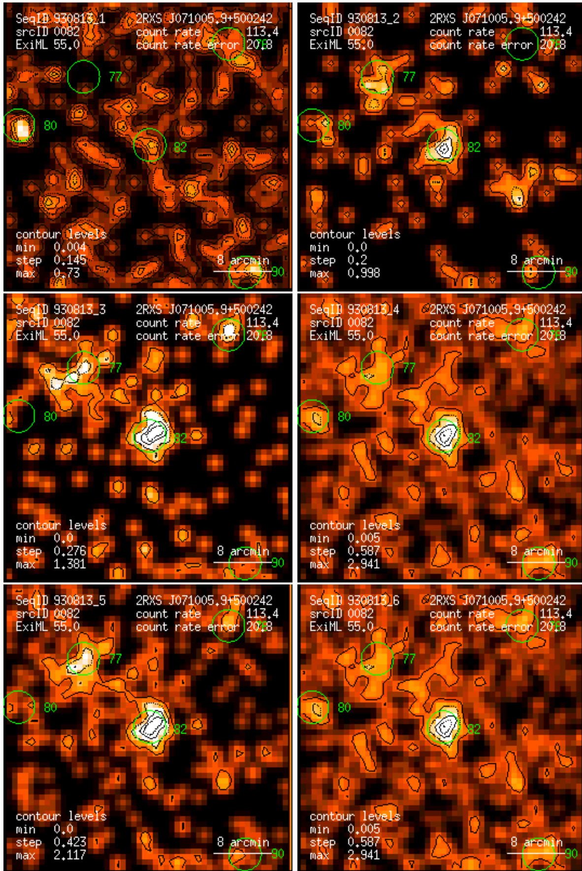
Figure 82: RASS 930813: detection 0082: band rate images, Gaussian filter: (1) PSPC channels 11 – 41, (2) 52 – 90, (3) 91 – 201, (4) 11 – 235, (5) 52 – 201, (6) 11 – 201. Broad band rates in counts/ks. Band rate contour levels in counts/ks/arcmin 2 .
