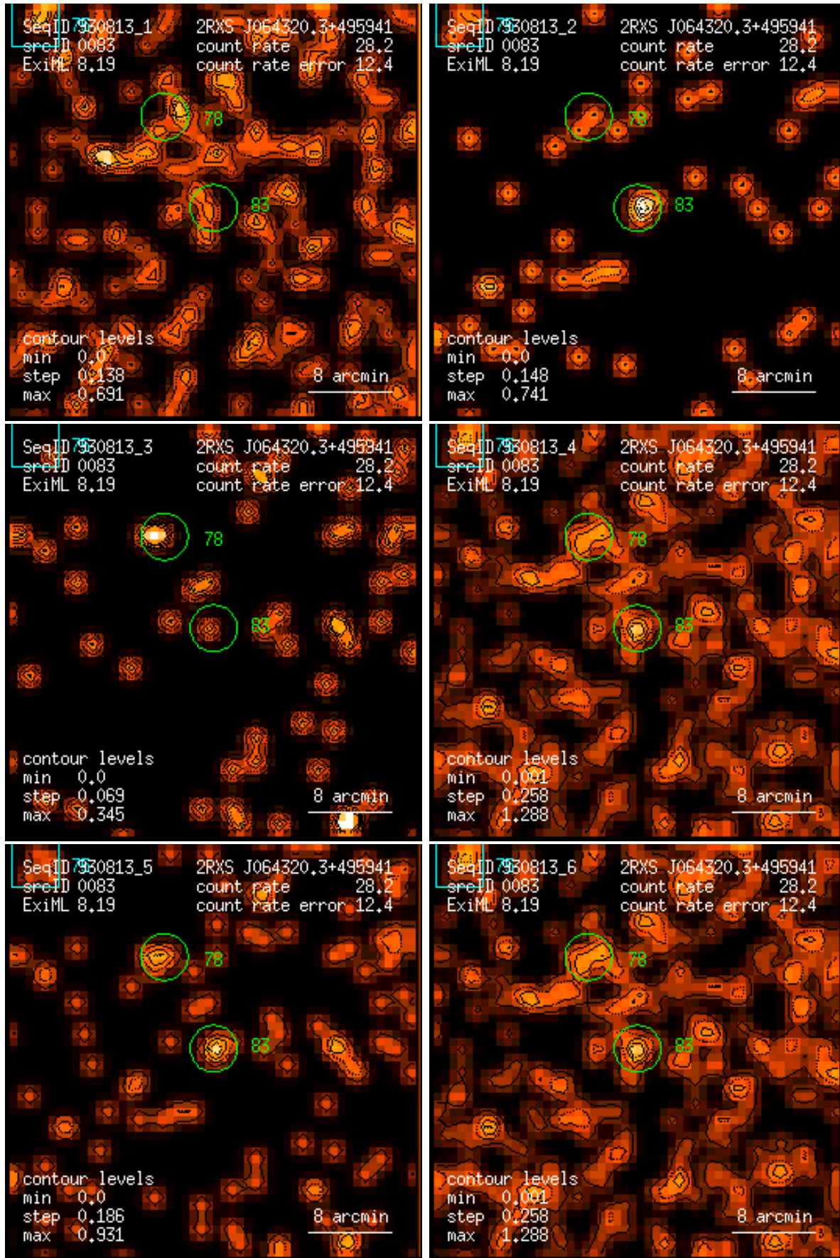
Figure 83: RASS 930813: detection 0083: band rate images, Gaussian filter: (1) PSPC channels 11 – 41, (2) 52 – 90, (3) 91 – 201, (4) 11 – 235, (5) 52 – 201, (6) 11 – 201. Broad band rates in counts/ks. Band rate contour levels in counts/ks/arcmin 2 .
