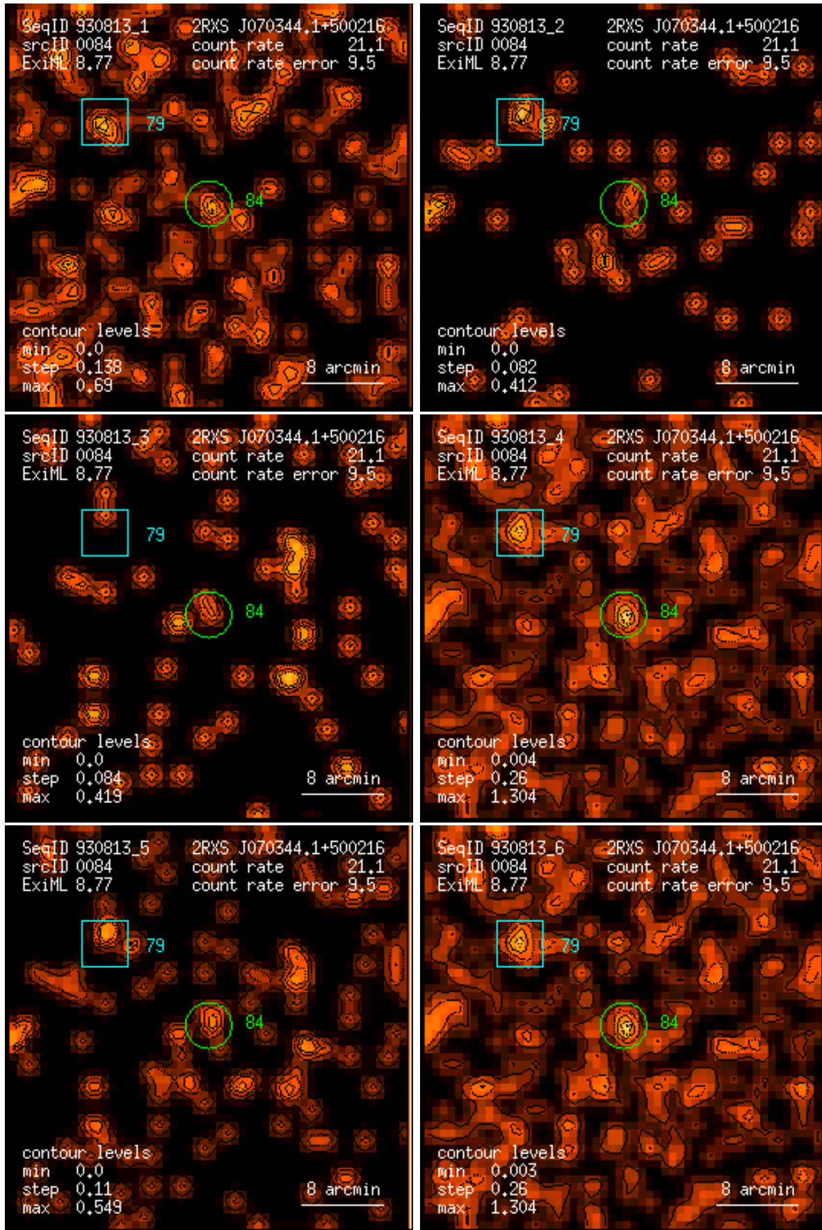
Figure 84: RASS 930813: detection 0084: band rate images, Gaussian filter: (1) PSPC channels 11 – 41, (2) 52 – 90, (3) 91 – 201, (4) 11 – 235, (5) 52 – 201, (6) 11 – 201. Broad band rates in counts/ks. Band rate contour levels in counts/ks/arcmin 2 .
