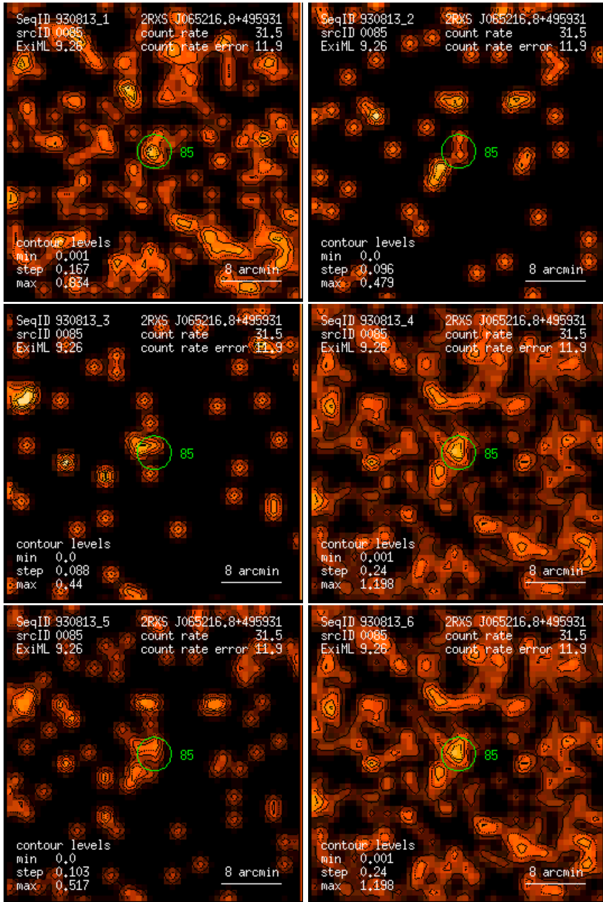
Figure 85: RASS 930813: detection 0085: band rate images, Gaussian filter: (1) PSPC channels 11 – 41, (2) 52 – 90, (3) 91 – 201, (4) 11 – 235, (5) 52 – 201, (6) 11 – 201. Broad band rates in counts/ks. Band rate contour levels in counts/ks/arcmin 2 .
