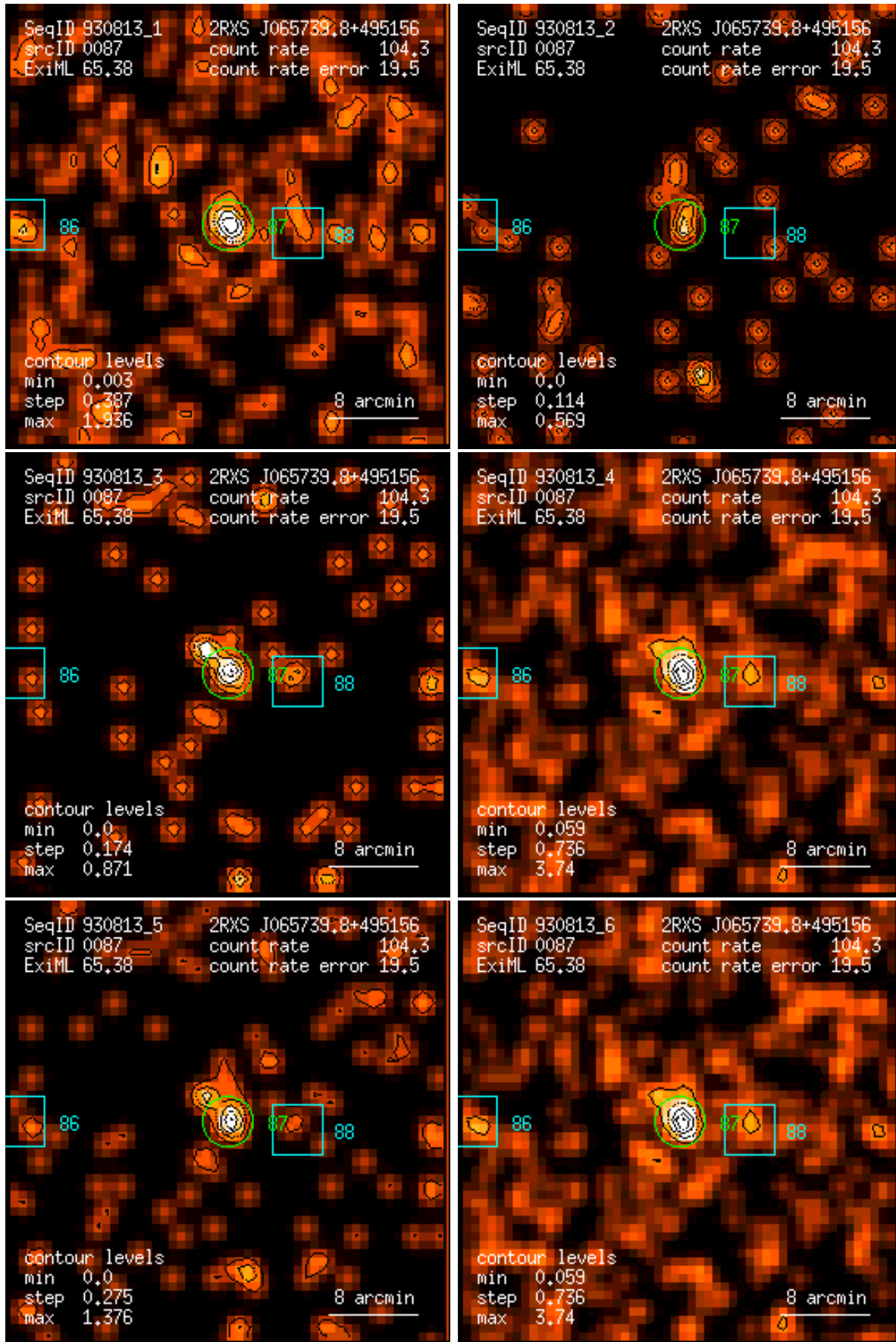
Figure 87: RASS 930813: detection 0087: band rate images, Gaussian filter: (1) PSPC channels 11 – 41, (2) 52 – 90, (3) 91 – 201, (4) 11 – 235, (5) 52 – 201, (6) 11 – 201. Broad band rates in counts/ks. Band rate contour levels in counts/ks/arcmin 2 .
