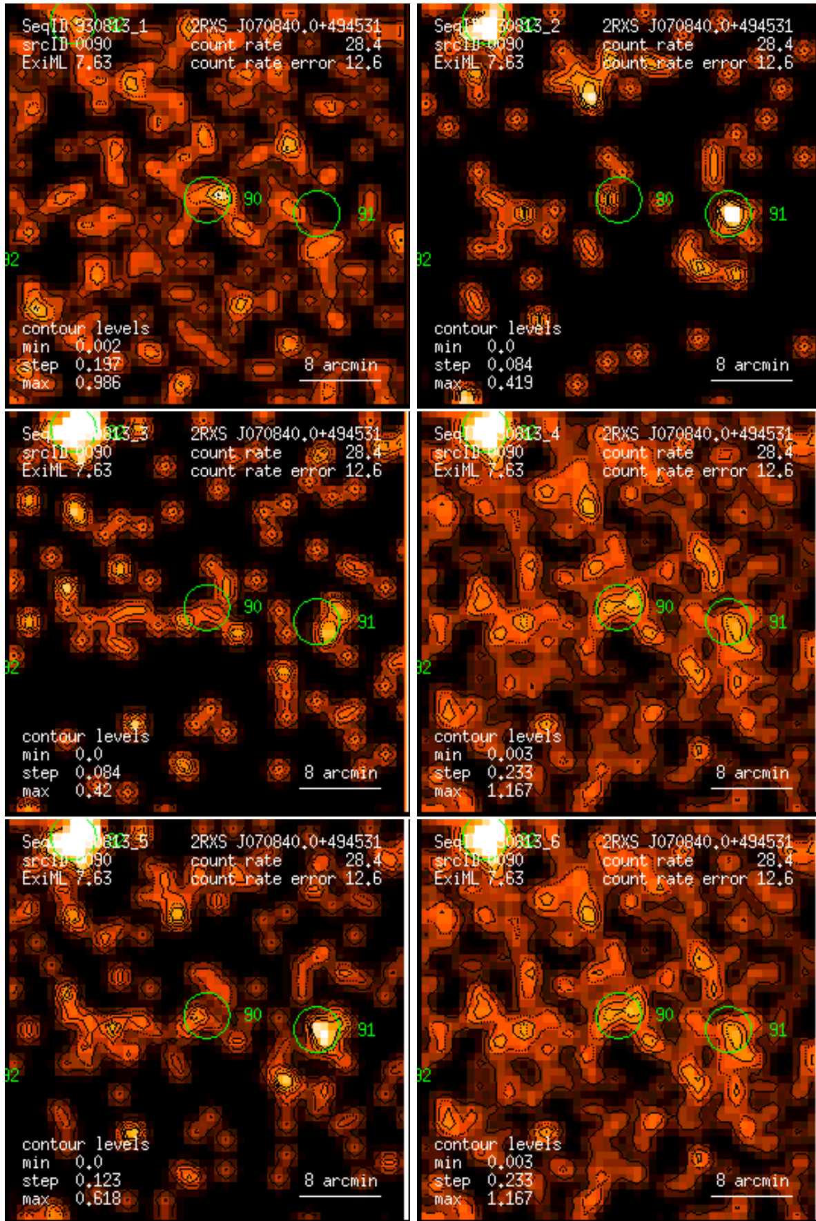
Figure 90: RASS 930813: detection 0090: band rate images, Gaussian filter: (1) PSPC channels 11 – 41, (2) 52 – 90, (3) 91 – 201, (4) 11 – 235, (5) 52 – 201, (6) 11 – 201. Broad band rates in counts/ks. Band rate contour levels in counts/ks/arcmin 2 .
