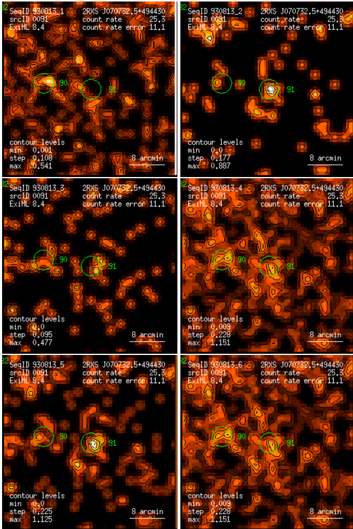
Figure 91: RASS 930813: detection 0091: band rate images, Gaussian filter: (1) PSPC channels 11 – 41, (2) 52 – 90, (3) 91 – 201, (4) 11 – 235, (5) 52 – 201, (6) 11 – 201. Broad band rates in counts/ks. Band rate contour levels in counts/ks/arcmin 2 .
