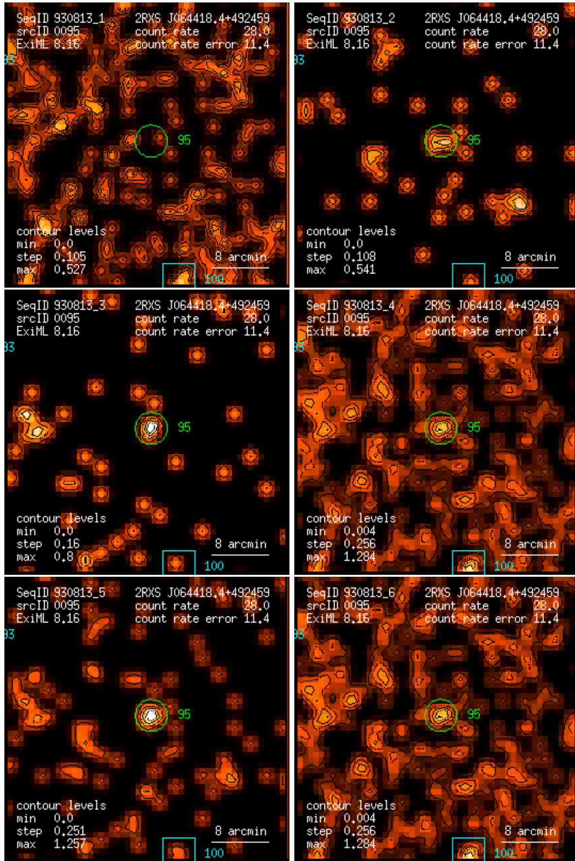
Figure 95: RASS 930813: detection 0095: band rate images, Gaussian filter: (1) PSPC channels 11 – 41, (2) 52 – 90, (3) 91 – 201, (4) 11 – 235, (5) 52 – 201, (6) 11 – 201. Broad band rates in counts/ks. Band rate contour levels in counts/ks/arcmin 2 .
