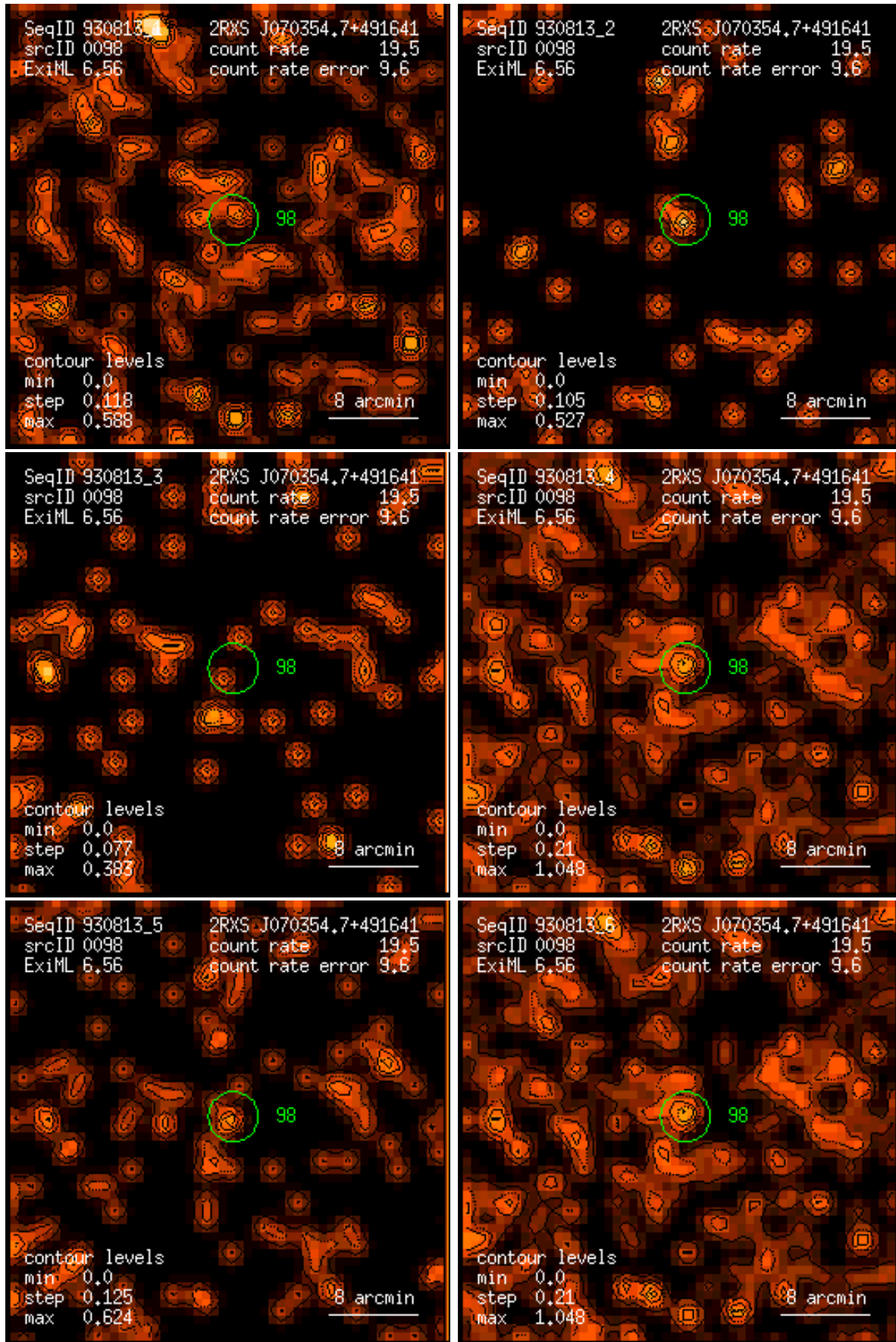
Figure 98: RASS 930813: detection 0098: band rate images, Gaussian filter: (1) PSPC channels 11 – 41, (2) 52 – 90, (3) 91 – 201, (4) 11 – 235, (5) 52 – 201, (6) 11 – 201. Broad band rates in counts/ks. Band rate contour levels in counts/ks/arcmin 2 .
