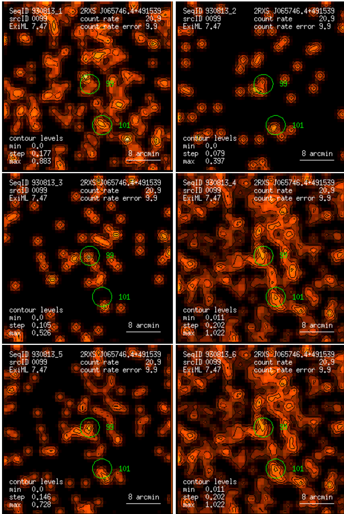
Figure 99: RASS 930813: detection 0099: band rate images, Gaussian filter: (1) PSPC channels 11 – 41, (2) 52 – 90, (3) 91 – 201, (4) 11 – 235, (5) 52 – 201, (6) 11 – 201. Broad band rates in counts/ks. Band rate contour levels in counts/ks/arcmin 2 .
