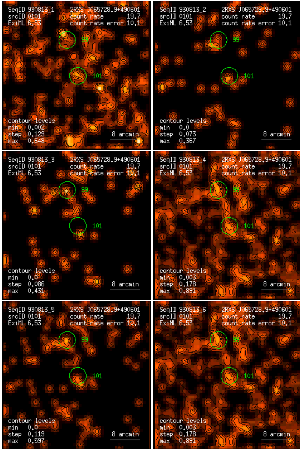
Figure 101: RASS 930813: detection 0101: band rate images, Gaussian filter: (1) PSPC channels 11 – 41, (2) 52 – 90, (3) 91 – 201, (4) 11 – 235, (5) 52 – 201, (6) 11 – 201. Broad band rates in counts/ks. Band rate contour levels in counts/ks/arcmin 2 .
