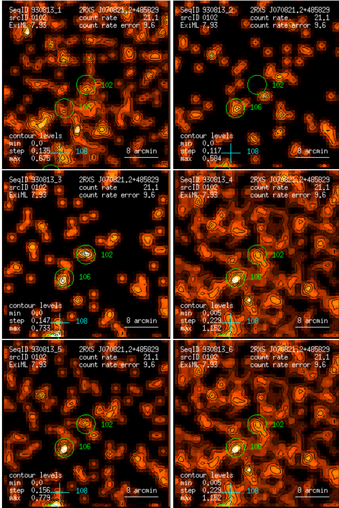
Figure 102: RASS 930813: detection 0102: band rate images, Gaussian filter: (1) PSPC channels 11 – 41, (2) 52 – 90, (3) 91 – 201, (4) 11 – 235, (5) 52 – 201, (6) 11 – 201. Broad band rates in counts/ks. Band rate contour levels in counts/ks/arcmin 2 .
