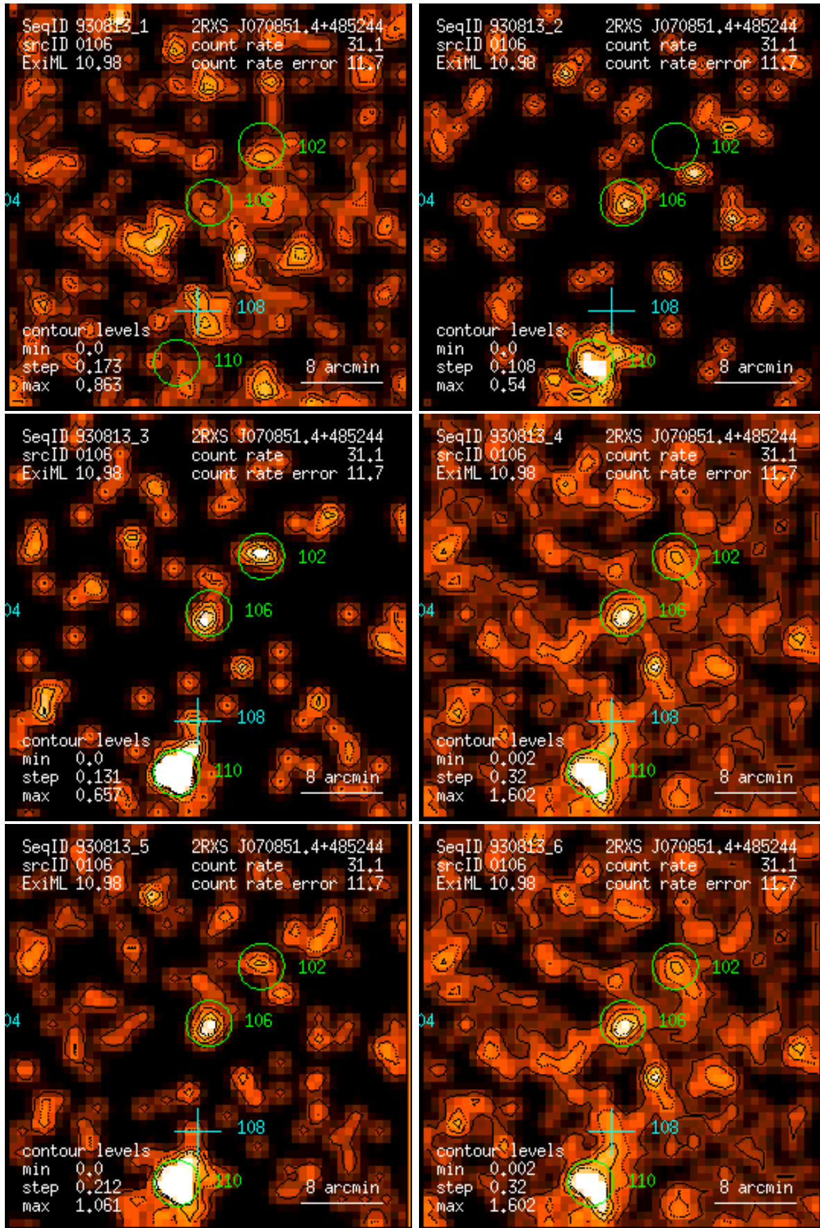
Figure 106: RASS 930813: detection 0106: band rate images, Gaussian filter: (1) PSPC channels 11 – 41, (2) 52 – 90, (3) 91 – 201, (4) 11 – 235, (5) 52 – 201, (6) 11 – 201. Broad band rates in counts/ks. Band rate contour levels in counts/ks/arcmin 2 .
