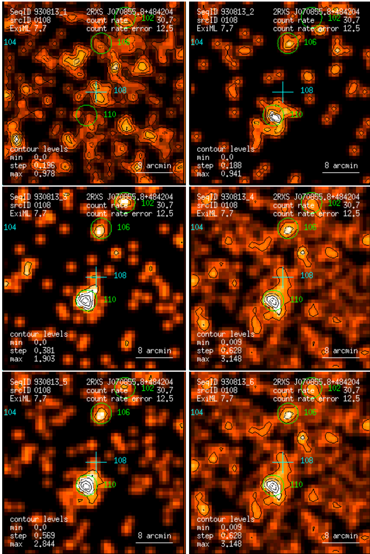
Figure 108: RASS 930813: detection 0108: band rate images, Gaussian filter: (1) PSPC channels 11 – 41, (2) 52 – 90, (3) 91 – 201, (4) 11 – 235, (5) 52 – 201, (6) 11 – 201. Broad band rates in counts/ks. Band rate contour levels in counts/ks/arcmin 2 .
