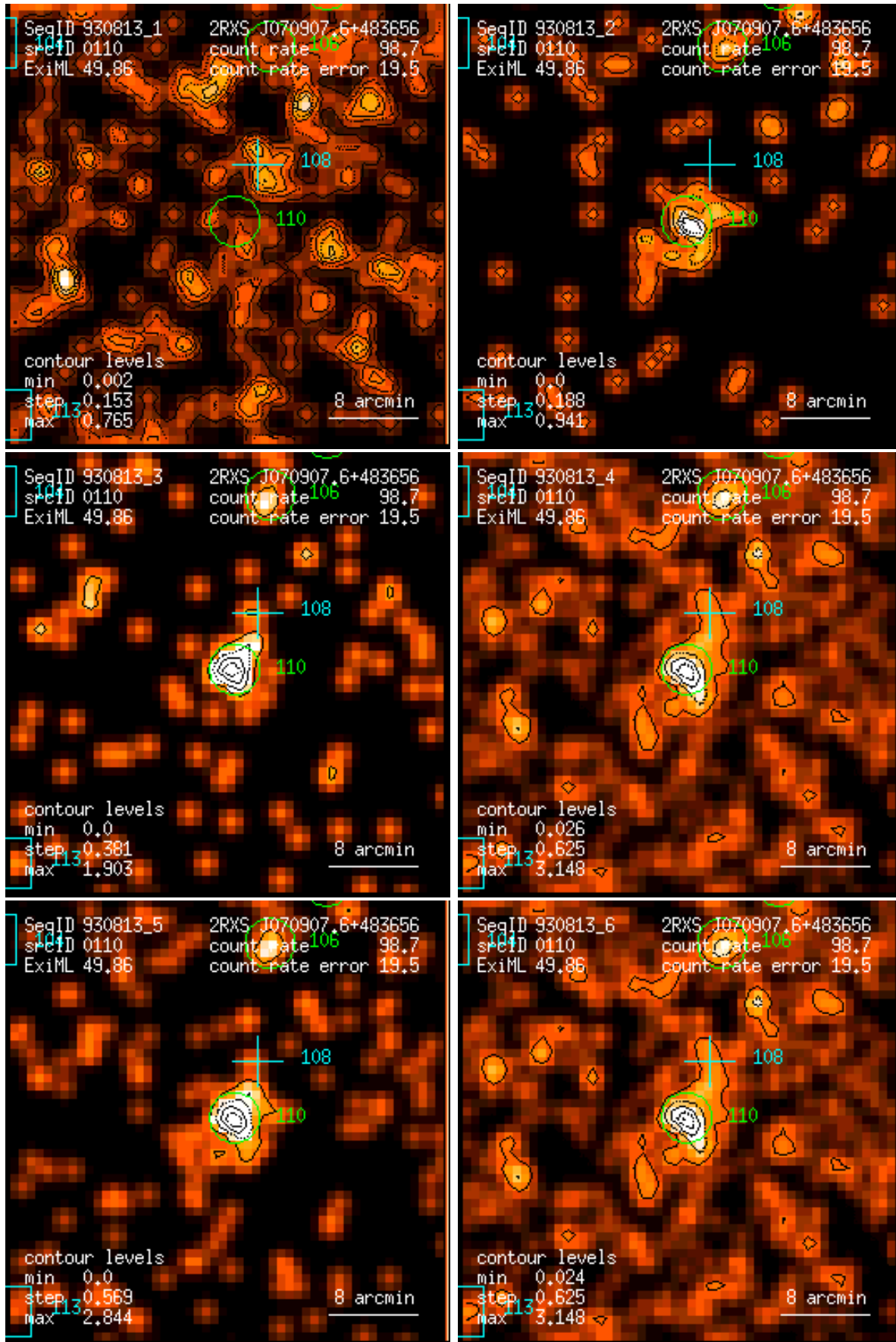
Figure 110: RASS 930813: detection 0110: band rate images, Gaussian filter: (1) PSPC channels 11 – 41, (2) 52 – 90, (3) 91 – 201, (4) 11 – 235, (5) 52 – 201, (6) 11 – 201. Broad band rates in counts/ks. Band rate contour levels in counts/ks/arcmin 2 .
