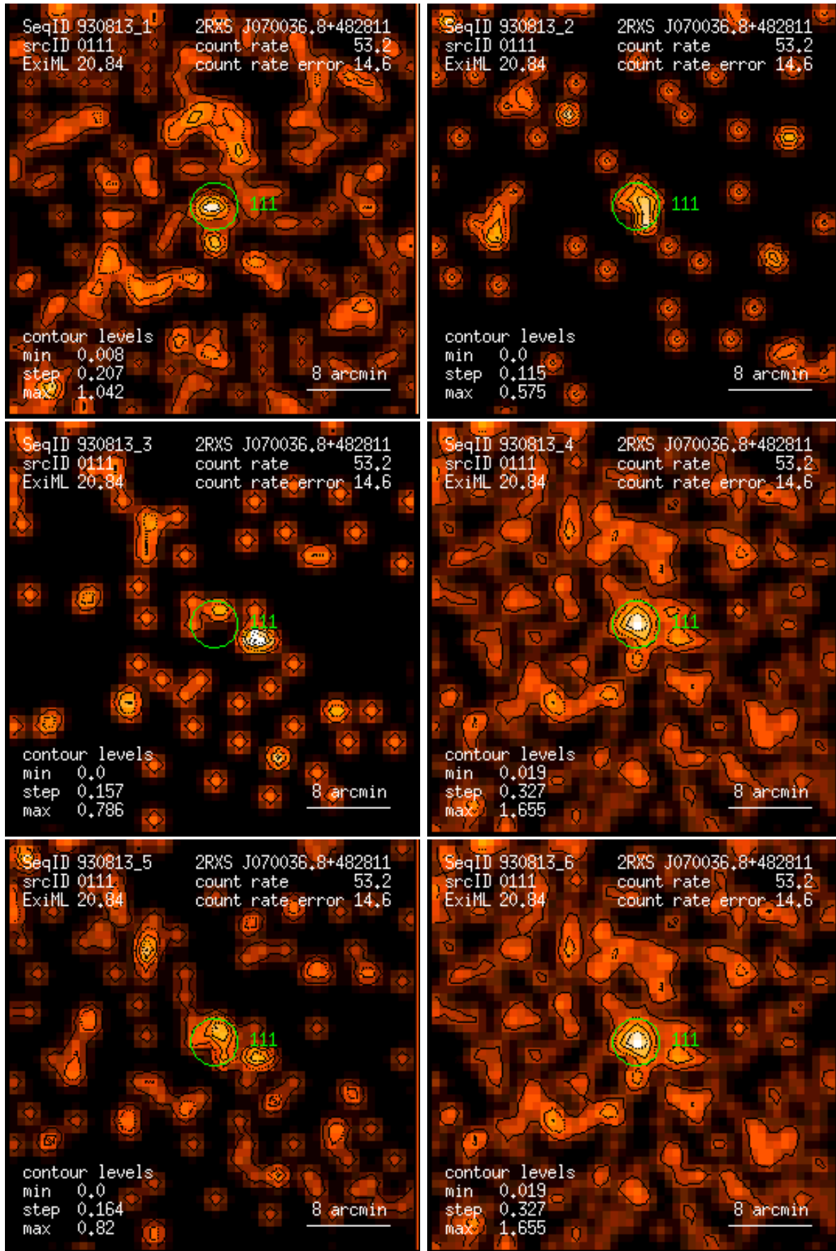
Figure 111: RASS 930813: detection 0111: band rate images, Gaussian filter: (1) PSPC channels 11 – 41, (2) 52 – 90, (3) 91 – 201, (4) 11 – 235, (5) 52 – 201, (6) 11 – 201. Broad band rates in counts/ks. Band rate contour levels in counts/ks/arcmin 2 .
