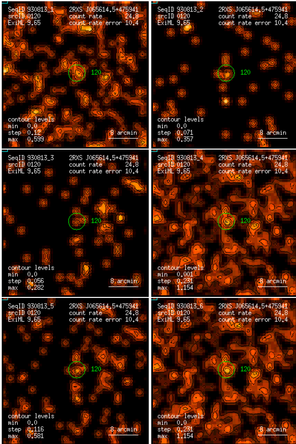
Figure 120: RASS 930813: detection 0120: band rate images, Gaussian filter: (1) PSPC channels 11 – 41, (2) 52 – 90, (3) 91 – 201, (4) 11 – 235, (5) 52 – 201, (6) 11 – 201. Broad band rates in counts/ks. Band rate contour levels in counts/ks/arcmin 2 .
