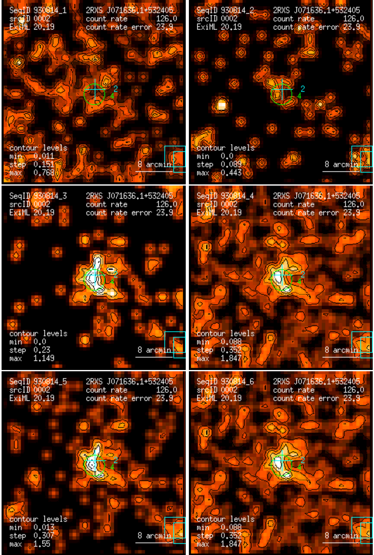
Figure 2: RASS 930814: detection 0002: band rate images, Gaussian filter: (1) PSPC channels 11 – 41, (2) 52 – 90, (3) 91 – 201, (4) 11 – 235, (5) 52 – 201, (6) 11 – 201. Broad band rates in counts/ks. Band rate contour levels in counts/ks/arcmin 2 .
