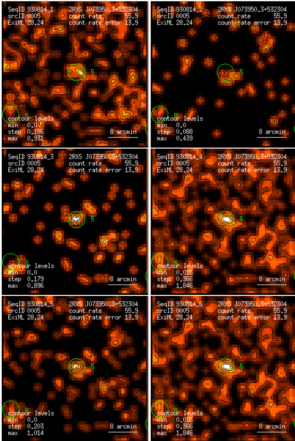
Figure 5: RASS 930814: detection 0005: band rate images, Gaussian filter: (1) PSPC channels 11 – 41, (2) 52 – 90, (3) 91 – 201, (4) 11 – 235, (5) 52 – 201, (6) 11 – 201. Broad band rates in counts/ks. Band rate contour levels in counts/ks/arcmin 2 .
