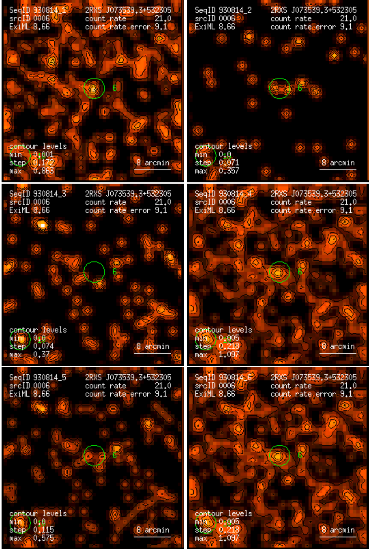
Figure 6: RASS 930814: detection 0006: band rate images, Gaussian filter: (1) PSPC channels 11 – 41, (2) 52 – 90, (3) 91 – 201, (4) 11 – 235, (5) 52 – 201, (6) 11 – 201. Broad band rates in counts/ks. Band rate contour levels in counts/ks/arcmin 2 .
