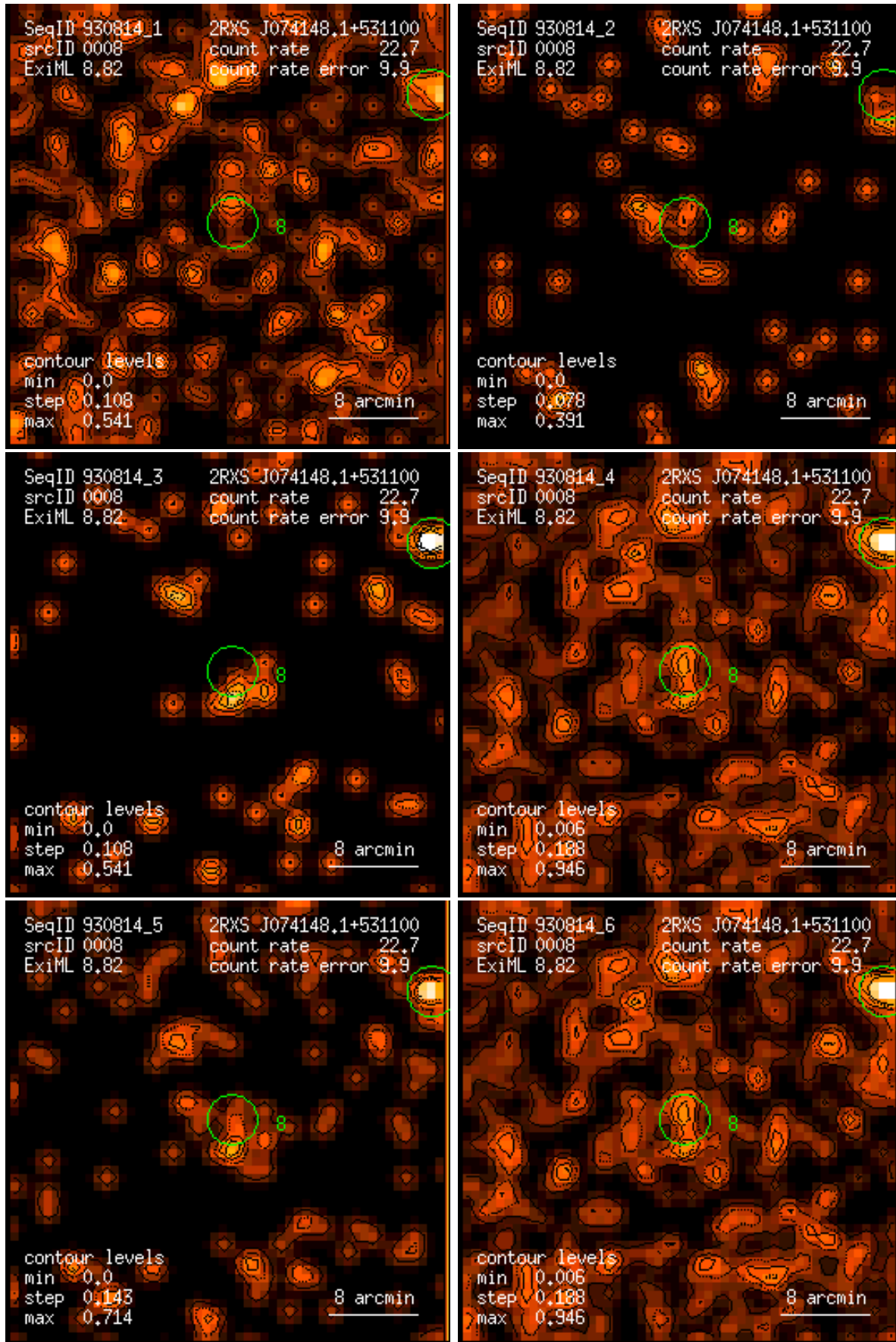
Figure 8: RASS 930814: detection 0008: band rate images, Gaussian filter: (1) PSPC channels 11 – 41, (2) 52 – 90, (3) 91 – 201, (4) 11 – 235, (5) 52 – 201, (6) 11 – 201. Broad band rates in counts/ks. Band rate contour levels in counts/ks/arcmin 2 .
