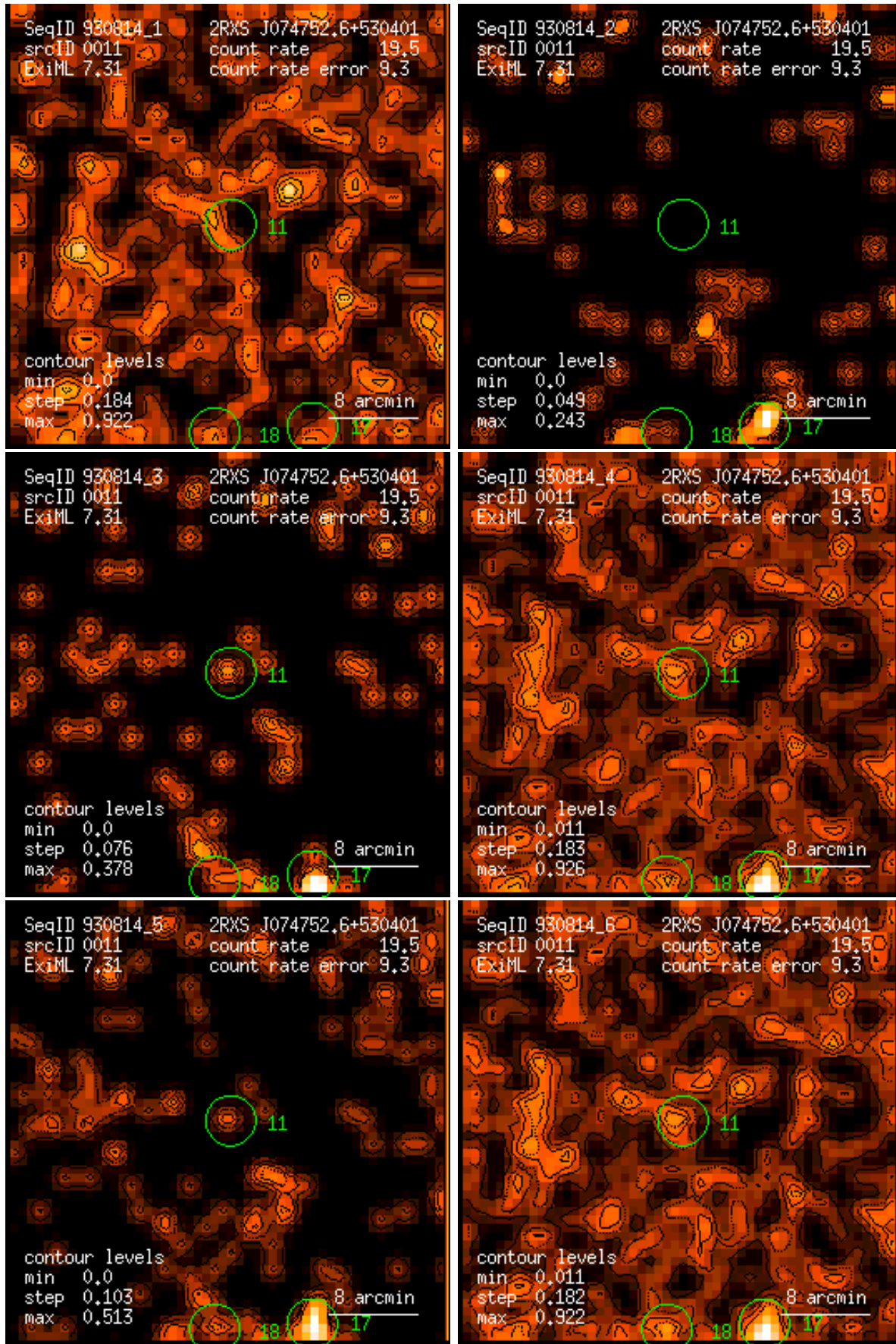
Figure 11: RASS 930814: detection 0011: band rate images, Gaussian filter: (1) PSPC channels 11 – 41, (2) 52 – 90, (3) 91 – 201, (4) 11 – 235, (5) 52 – 201, (6) 11 – 201. Broad band rates in counts/ks. Band rate contour levels in counts/ks/arcmin 2 .
