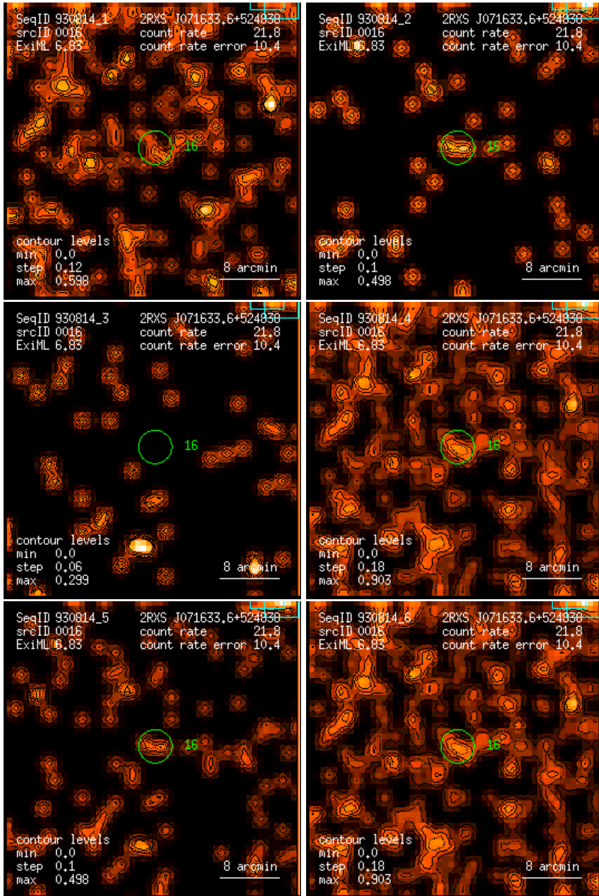
Figure 16: RASS 930814: detection 0016: band rate images, Gaussian filter: (1) PSPC channels 11 – 41, (2) 52 – 90, (3) 91 – 201, (4) 11 – 235, (5) 52 – 201, (6) 11 – 201. Broad band rates in counts/ks. Band rate contour levels in counts/ks/arcmin 2 .
