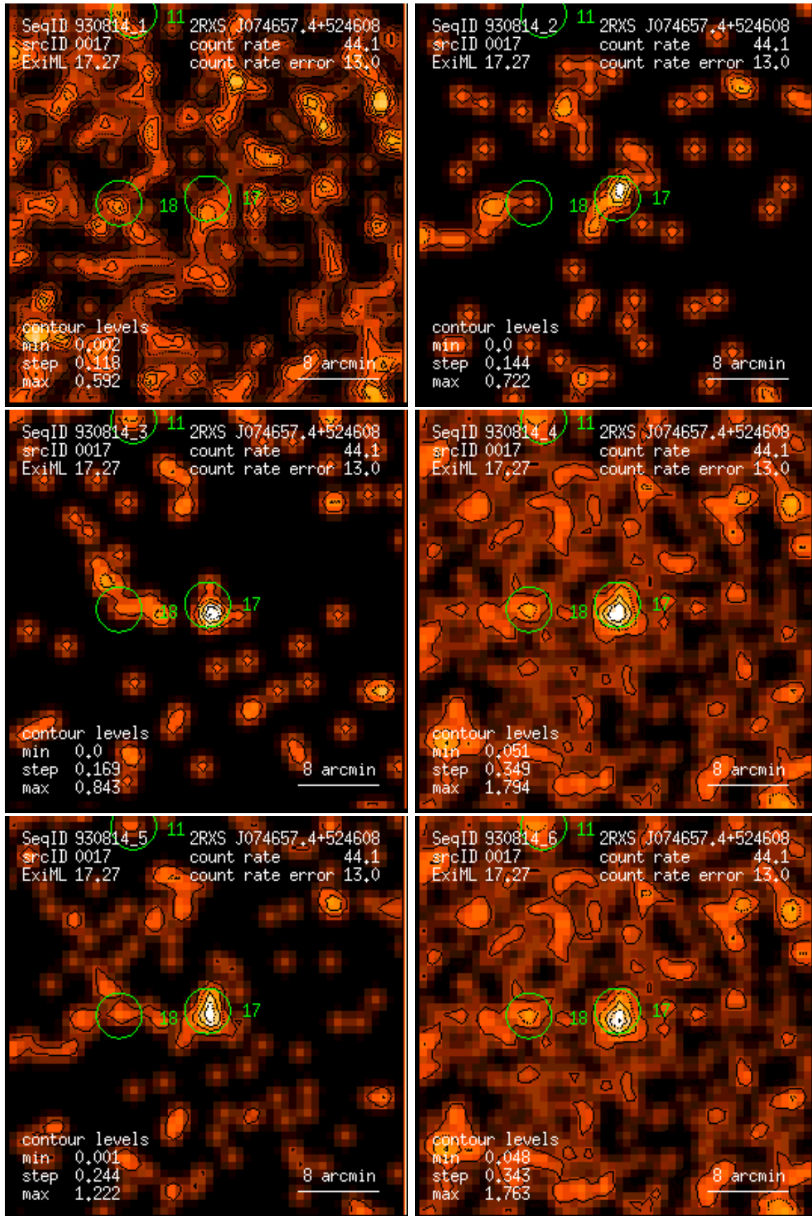
Figure 17: RASS 930814: detection 0017: band rate images, Gaussian filter: (1) PSPC channels 11 – 41, (2) 52 – 90, (3) 91 – 201, (4) 11 – 235, (5) 52 – 201, (6) 11 – 201. Broad band rates in counts/ks. Band rate contour levels in counts/ks/arcmin 2 .
