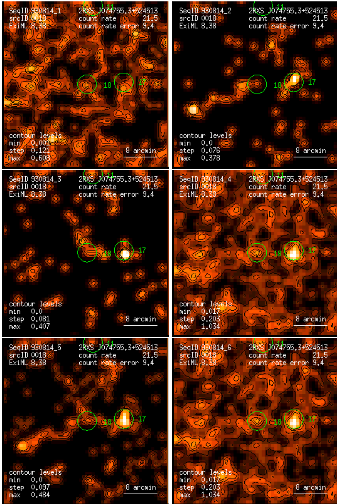
Figure 18: RASS 930814: detection 0018: band rate images, Gaussian filter: (1) PSPC channels 11 – 41, (2) 52 – 90, (3) 91 – 201, (4) 11 – 235, (5) 52 – 201, (6) 11 – 201. Broad band rates in counts/ks. Band rate contour levels in counts/ks/arcmin 2 .
