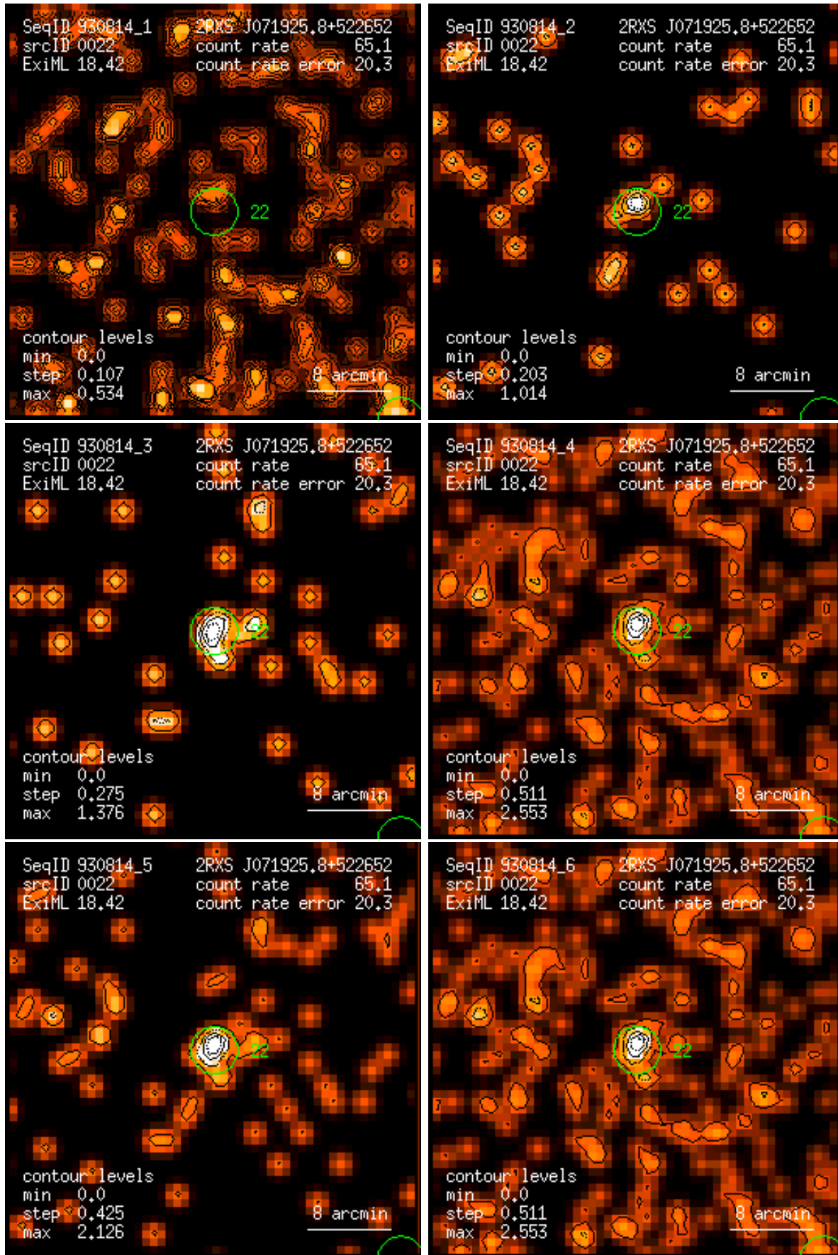
Figure 22: RASS 930814: detection 0022: band rate images, Gaussian filter: (1) PSPC channels 11 – 41, (2) 52 – 90, (3) 91 – 201, (4) 11 – 235, (5) 52 – 201, (6) 11 – 201. Broad band rates in counts/ks. Band rate contour levels in counts/ks/arcmin 2 .
